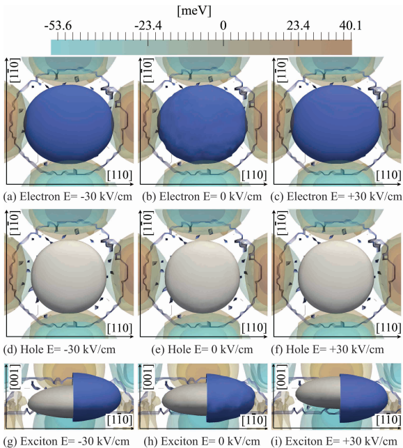
FIG. 4. Single quantum dot. Volumetric cross-section of electron and hole charge distributions with and without the applied vertical ( [001] ) electric field. We include isosurfaces of the piezoelectric potential and the outline of the quantum dot structure. In panels (a)-(f) the horizontal extent corresponds to the [110] direction and the vertical one to the [1\bar{1}0] direction. In panels (g)-(i) the height of picture represents the [001] direction and the width [1\bar{1}0] direction, and for clarity the hole isosurface is shown on the left (grey) and electron isosurface on the right (blue).
