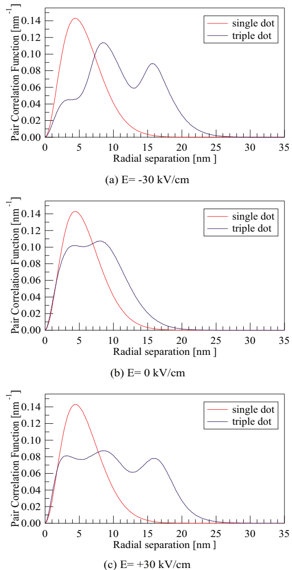
FIG. 6. Pair correlation function for the single and triple quantum dots for three electric field values.
