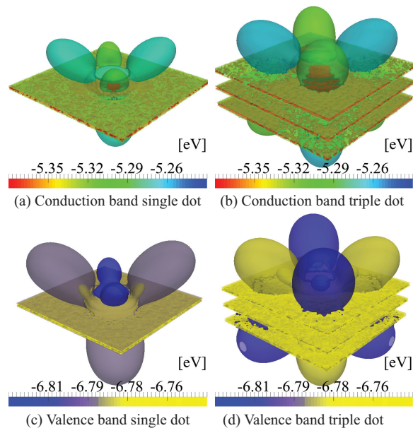
FIG. 3. Strain and piezoelectric field modified conduction and valence band the model quantum dots.
