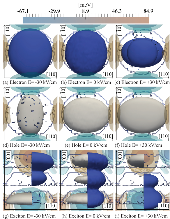
FIG. 5. Coupled quantum dot. Volumetric cross-section of electron and hole charge distributions with and without the applied vertical ( [001] ) electric field. We include isosurfaces of the piezoelectric potential and the outline of the quantum dot structure. In panels (a)-(f) the horizontal extent corresponds to the [110] direction and the vertical one to the [1\bar{1}0] direction. In panels (g)-(i) the height of picture represents the [001] direction and the width [1\bar{1}0] direction, and for clarity the hole isosurface is shown on the left (grey) and electron isosurface on the right (blue).
