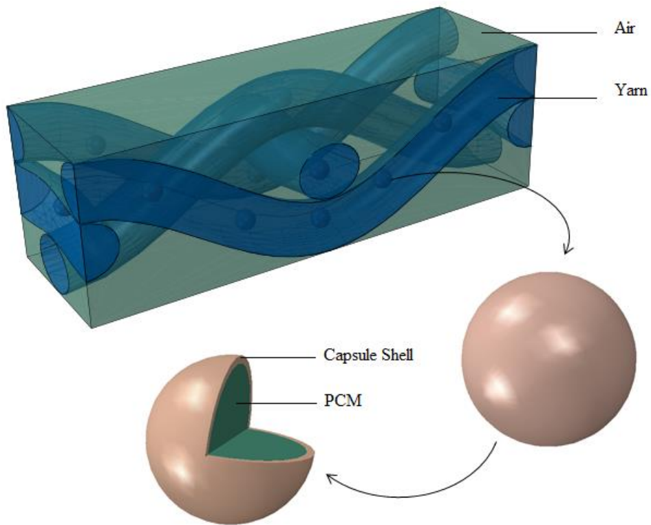
Figure 14 Geometric model
