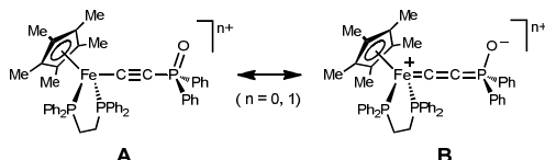
Scheme 3: Valence bond representation of 3a .
