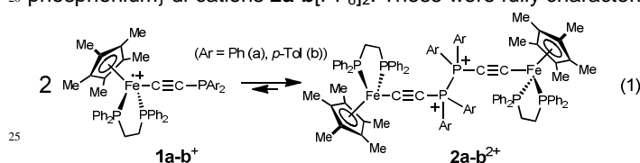
Scheme 1: Equilibrium between the Fe(III) monomer 1 [PF 6 ] and the corresponding bis-Fe(II) dimer 2 [PF 6 ] 2
