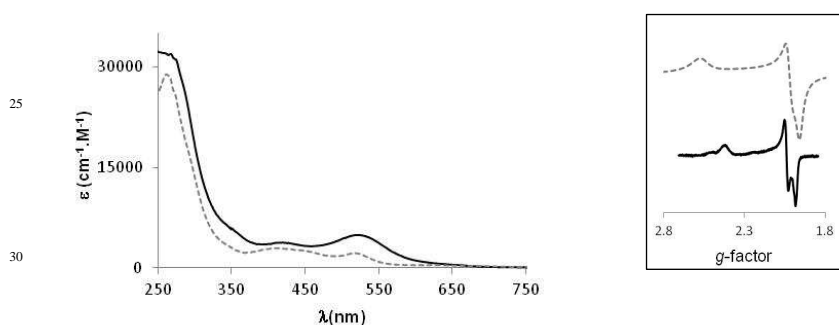
Fig 3. Overlay of the UV-vis spectra of 10^{-5} M solutions of \mathbf{2a}[\text{PF}_6]_2 (plain line) and \mathbf{3a}[\text{PF}_6] (dotted line) in \text{CH}_2\text{Cl}_2 at 298 K. Inset: ESR spectra of frozen solutions of \mathbf{2a}[\text{PF}_6]_2 (plain line) and \mathbf{3a}[\text{PF}_6] (dotted line) in \text{CH}_2\text{Cl}_2/1,2\text{-C}_2\text{H}_4\text{Cl}_2 solvent glasses at 77K.
