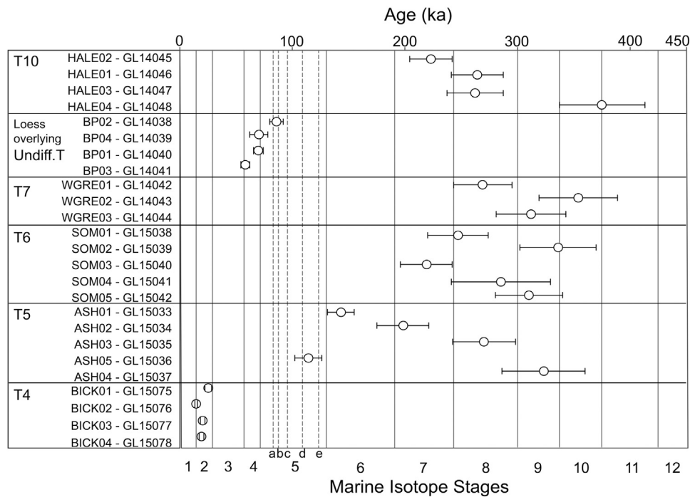
Fig. 10. Summary diagram showing OSL age estimates from the eastern Solent terraces in relation to the Marine Isotope stratigraphy, after LR04 (Lisiecki and Raymo, 2005).
