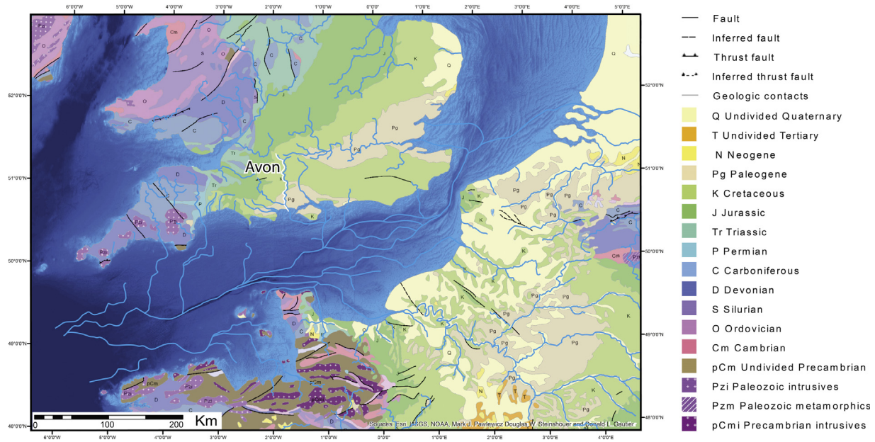
Fig. 1. Map showing the bedrock geology and Pleistocene rivers of southern Britain and northwest Europe (Sources: Esri, USGS, NOAA, M. J. Pawlewicz, D.W. Steinhauer and D. L. Gautier. Bathymetric data: GEBCO_2014 Grid, version 20141103, http://www.gebco.net ) (Data in the map were modelled by LB in ArcGIS 10.5 under licence to Queen's University Belfast).
