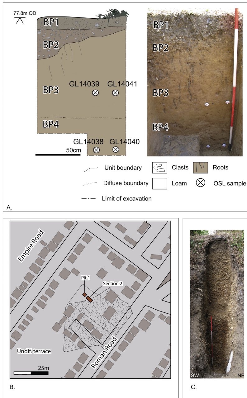
Fig. 3. A. South east section of pit 1 at Bemerton showing the massive loess found overlying the river gravels and the four OSL sample locations. B. OS map of Bemerton visualising the location of Pit 1, on top of the terrace and behind Section 2. C. Photograph of Section 2 1:10000 scale OS VectorMap Local [shape file], Digimap Licence.
