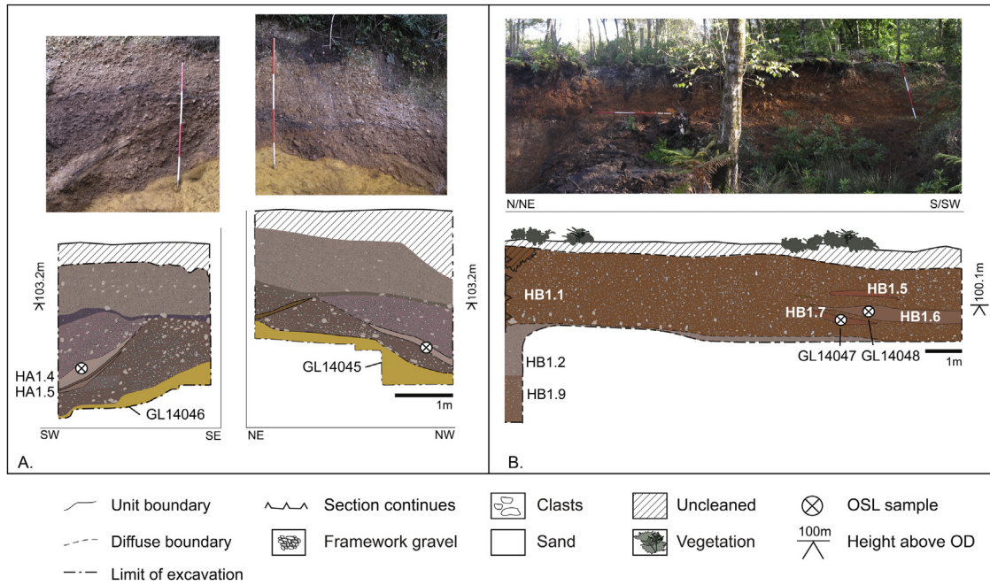
Fig. 4. A. South and north section of Hatchet Gate Farm gravel pit. B. West section of Woodriding gravel pit.
