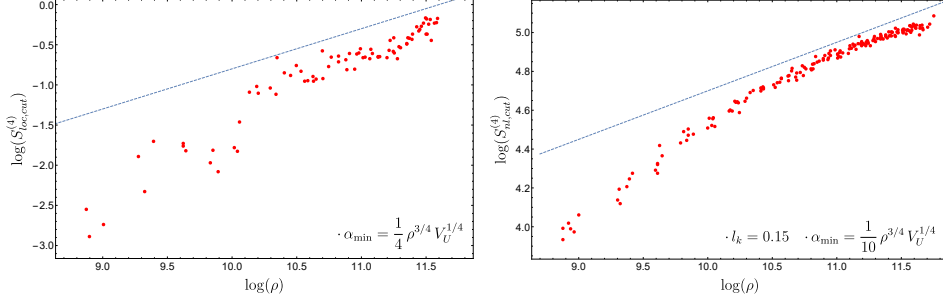
Figure 5: Entanglement entropy vs. number of points in the subregion U for the local (left) and nonlocal (right) theories with cutoffs on both the global Wightman function, W , and W_\kappa|_U . The blue dashed lines have slopes \rho^{1/2} (left) and \rho^{1/4} (right), they correspond to the “area-law” scaling expected in the local theory and nonlocal theory (as for Eq. (32)) respectively.
