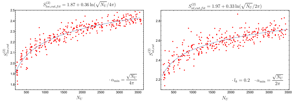
Figure 3: Entanglement entropy vs. number of points in the subregion U for the local (left) and nonlocal (right) theories with cutoffs on both the global Wightman function, W , and W_\kappa|_U .
