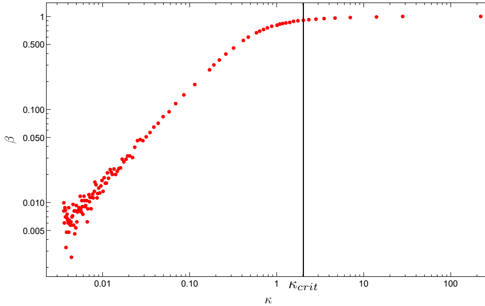
Figure 10: A plot of \beta vs. \kappa . Note that for large \kappa > \kappa_{crit} the value of \beta is approximately constant and close to 1. As \kappa decreases below \kappa_{crit} the value of \beta starts decreasing rapidly. This implies that for values of 0 < \kappa \ll \kappa_{crit} valid Cauchy regions must be large, while for \kappa_{crit} \gtrsim \kappa < 1 they can be relatively small. Note also that \kappa_{crit} corresponds roughly to the point in the spectrum of i\Delta just before the kink.
