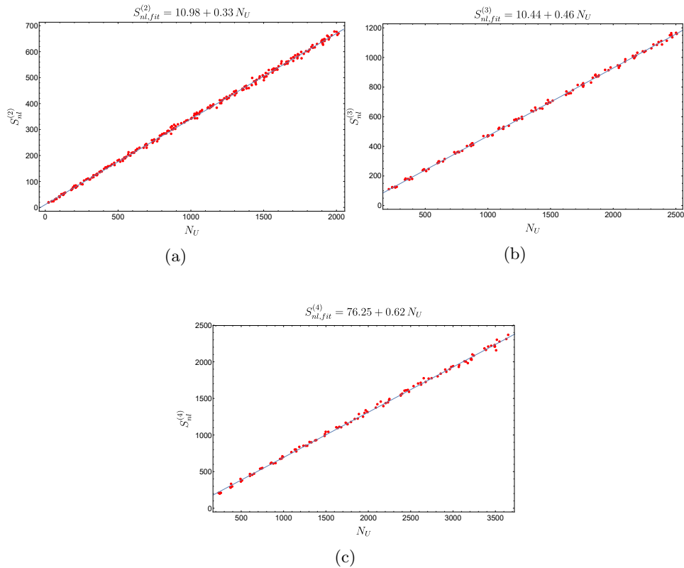
Figure 8: Finite part of the entanglement entropy vs. number of points in the subregion U for d=2 (left), 3 (right) and 4 (bottom), in the nonlocal case. This finite contribution is obtained by matching the kernel of R to the one of \Delta and follows a spacetime volume law.
