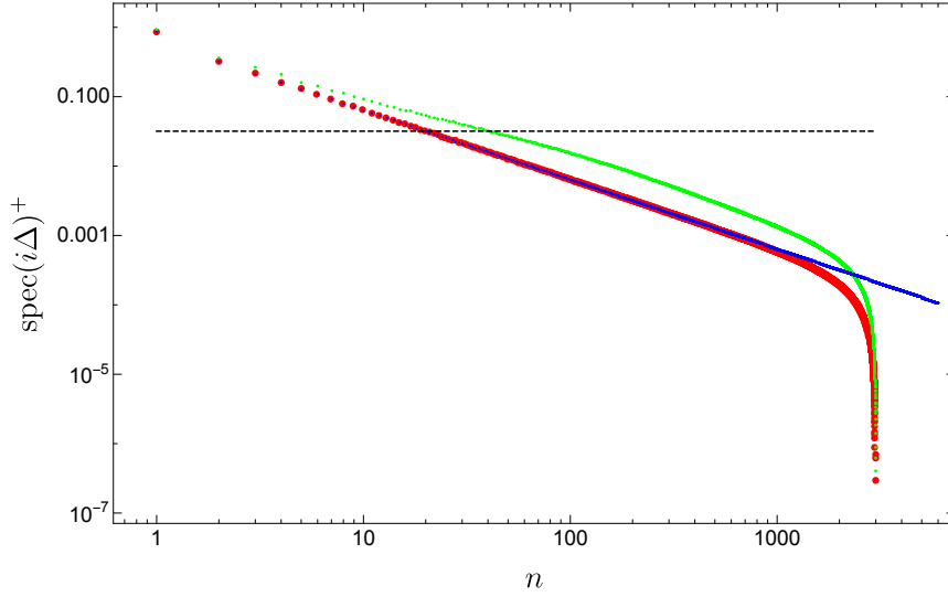
Figure 2: Positive part of \text{spec}(i\Delta) for a diamond in Minkowski spacetime for both a sprinkling of the diamond (in red for the local theory and green for the nonlocal theory) and in the continuum (in blue). The eigenvalues have been ordered by size from largest to smallest. The red line represents the case discussed in the previous section of a local Pauli–Jordan function, the blue line is the spectrum of the continuum theory and the green one represents the spectrum of the nonlocal Pauli–Jordan function with l_k = 0.2 . The black, dashed line signals the end of the strictly infrared spectrum and the onset of the nonlocal regime.
