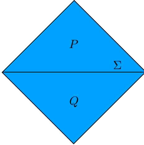
Figure 9: Causal diamond in \mathbb{M}^2 with Cauchy surface \Sigma . P and Q are the future and past domains of dependence of \Sigma respectively.
