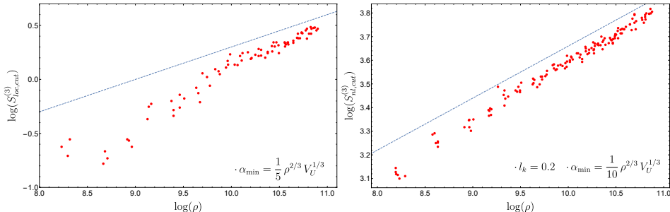
Figure 4: Entanglement entropy vs. number of points in the subregion U for the local (left) and nonlocal (right) theories with cutoffs on both the global Wightman function, W , and W_\kappa|_U . The blue dashed lines have slopes \rho^{1/3} (left) and \rho^{2/9} (right), they correspond to the “area-law” scaling expected in the local theory and in the nonlocal theory (as for Eq. (32)) respectively.
