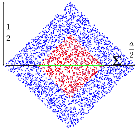
Figure 1: Inner and outer diamonds for a sprinkling in 2d Minkowski, with N = 2048 and V/V_U = 4 . The Sorkin entropy S(\mathcal{C}_U) is the causet analogue of the entanglement entropy of the vacuum state on \Sigma restricted to the interior of the diamond.
