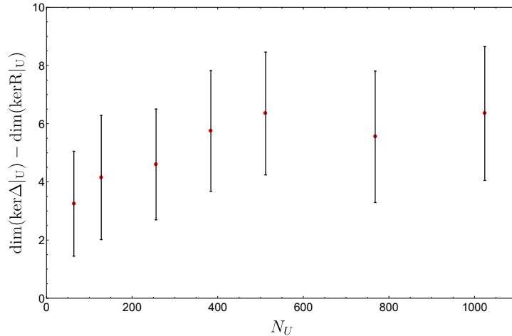
Figure 6: Plot of the average difference between \ker \Delta|_U and \ker R|_U .
