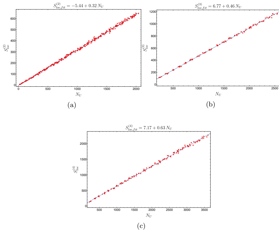
Figure 7: Finite part of the entanglement entropy vs. number of points in the subregion U for d=2 (left), 3 (right) and 4 (bottom). This finite contribution is obtained by matching the kernel of R to the one of \Delta and follows a spacetime volume law.
