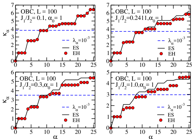
FIG. 22. Ratio \kappa_{\alpha}s for the J_1 - J_2 chain with OBC. The black solid line and red circles stands for ratios computed from the exact ES and the EH spectrum respectively. The blue dashed line marks \rho_A eigenvalues with a magnitude indicated in the legend. Agreement with BW theorem is good in the middle of the critical phase and close to it (relative deviations smaller than 10%), while it gets worse as J_2/J_1 is increased away from the critical line (relative deviations larger than 20%).
