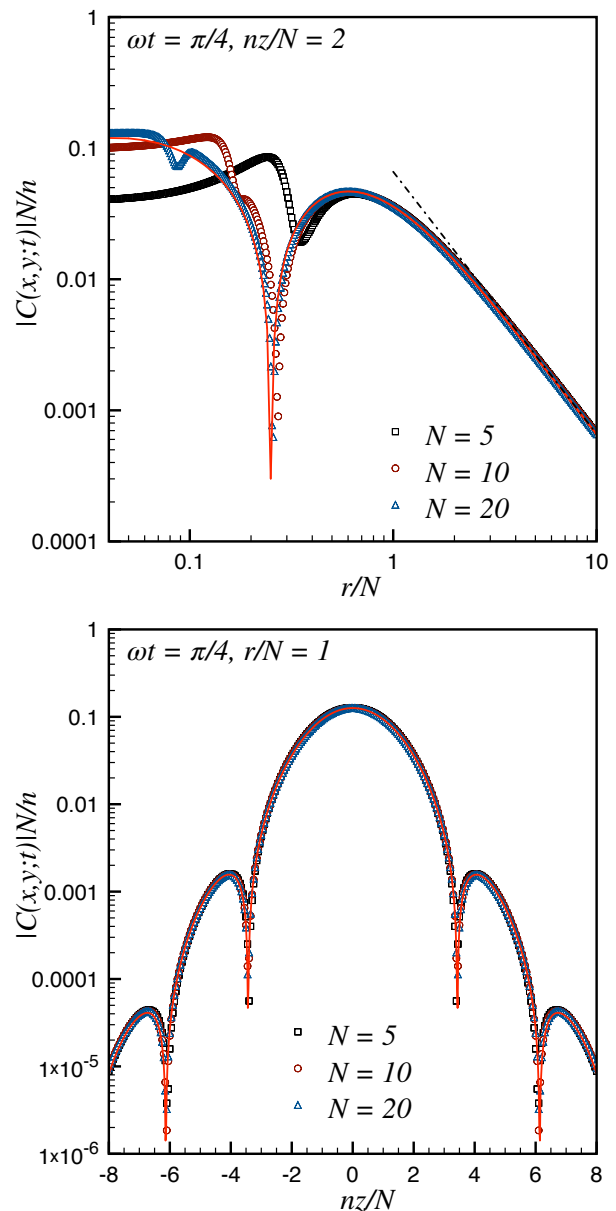
FIG. 2: Fermionic correlation function at fixed time \omega t = \pi/4 as a function of the distance r from the center of the trap at fixed separation z (top panel) and the other way around (bottom panel). The symbols are the exact data at finite N (the apparent singularities are just sign changes in logarithmic scale). The full red line in the top (bottom) panel is the large r asymptotics in Eq. (33) (Eq. (34)), where the first twenty terms in the sum have been kept. The dot-dashed line in the left panel is the very large r algebraic tail, i.e. the first term of Eq. (34).
