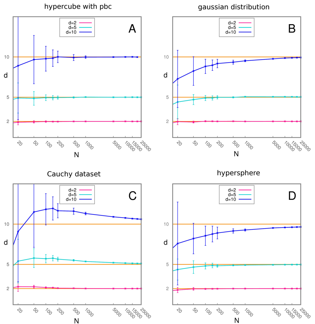
Figure 2. Scaling of the estimated ID with respect to the number of points; for each distribution and for a number of points going from 20 to 25000 we harvest 200 instances of the dataset and average the resulting estimates for the ID. The test is carried out in dimension 2, 5 and 10. Panel A: Hypercube with pbc. Panel B: gaussian distribution. Panel C: Cauchy dataset. Panel D: uniform distribution on a hypersphere.
