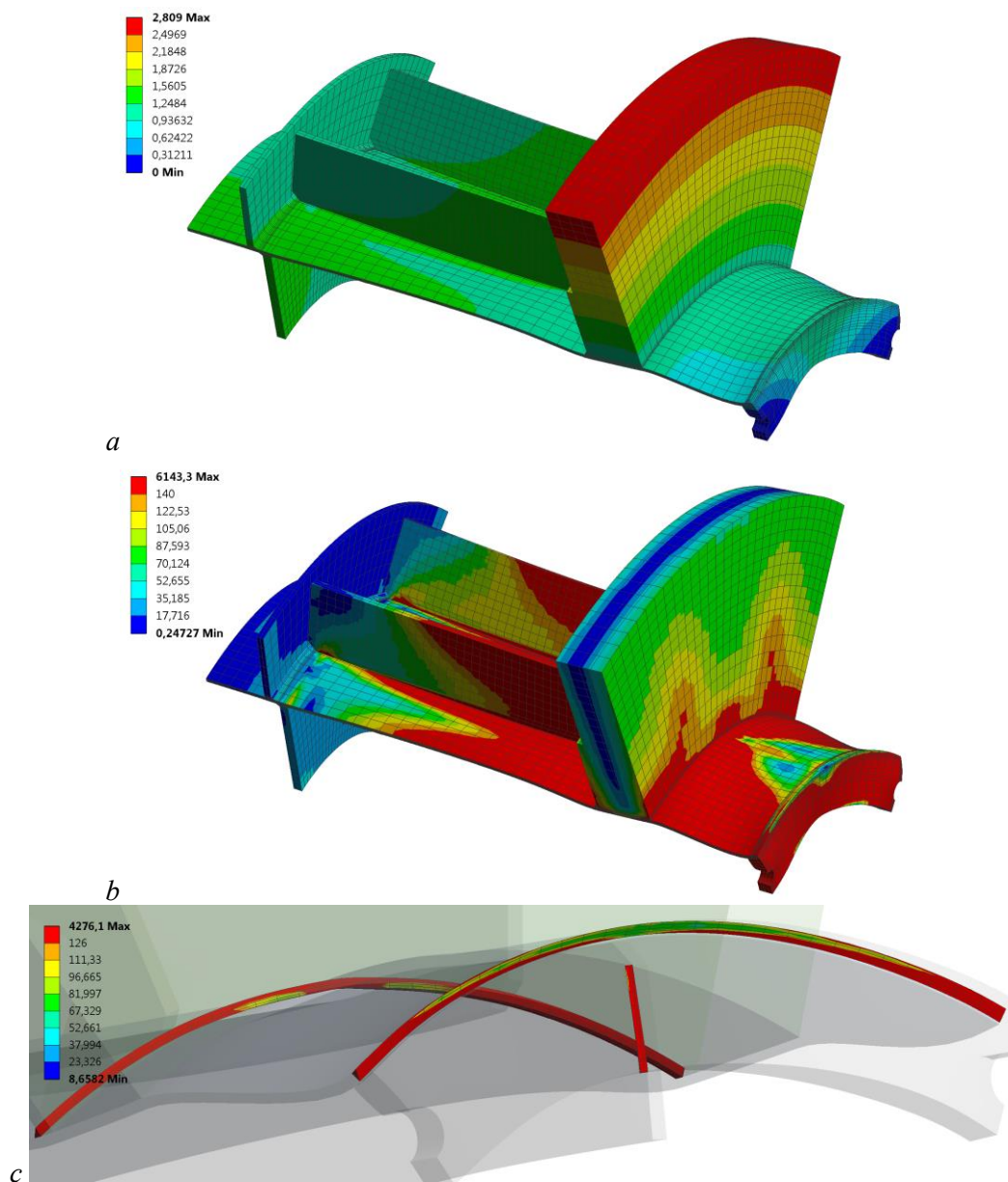
Figure 3. Stress-strain behavior of DN 1200 sealer device under static load: a – total displacements (scaled up), mm; b – von Mises stress, MPa; c – von Mises stress in most loaded welded joints, MPa.
