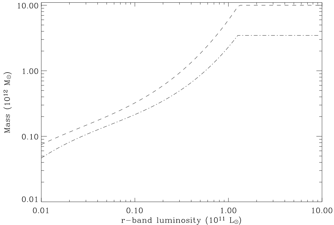
Figure 1: The conversion from galaxy luminosity to galaxy halo mass. Dashed line: early-type galaxies; dash-dotted line: late-type galaxies.
