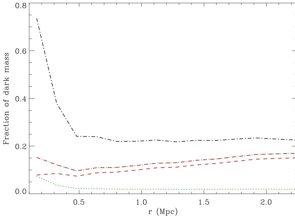
Figure 3: The ratio of the baryonic to the DM profiles. Green dotted line: (baryons in galaxies)/DM; red dashed line: (IC gas baryons)/DM; green and red dash-dotted line: (all baryons)/DM. The ratio of the subhaloes mass profile to the DM profile is shown as a black dash-dotted line.
