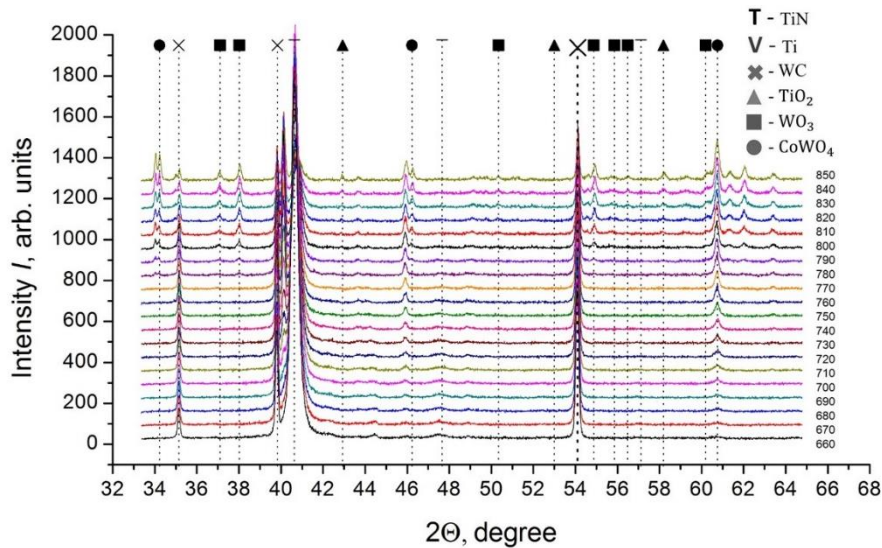
Figure 3. Diffraction pattern of a Ti–Cu–N coating at in situ thermal influence in open air up to 850\text{ }^\circ\text{C} (660–850 ^\circ\text{C} ).
