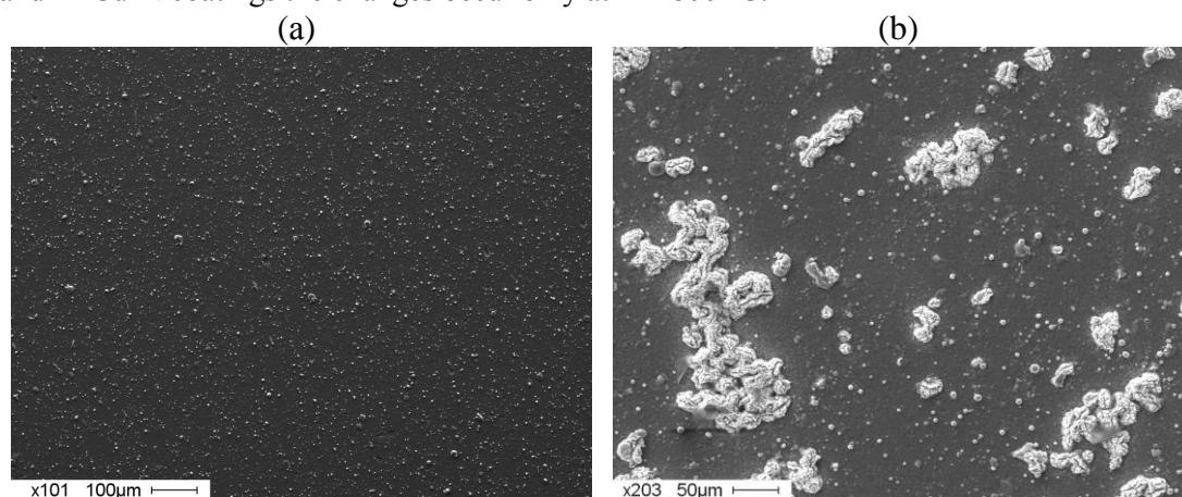
Figure 1. SEM images of specimen with deposited Ti-Cu-N coatings before (a) and after (b) high-temperature oxidation in open air at temperature of 850-850 °C.
