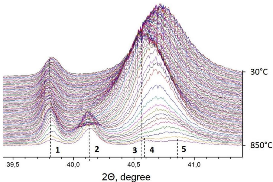
Figure 4. Diffraction pattern ( 2\theta = 39.4 - 41.4\text{ }^\circ ) of a Ti–Cu–N coating at in situ thermal influence in open air up to 850\text{ }^\circ\text{C} (30 – 850\text{ }^\circ\text{C} , inverse temperature dependence): 1 – WC; 2 – \text{TiO}_2 ; 3 – TiN; 4 – \text{WO}_3 ; 5 – \text{TiO}_2 .
