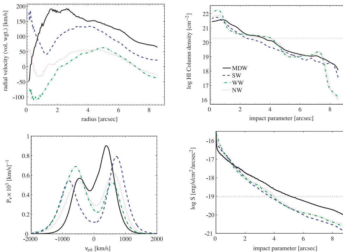
Figure 5. Angularly averaged properties of Halo 1, for the wind prescriptions shown in the legend (upper left), as discussed in Section 4.3. The upper-left panel shows the volume-averaged radial velocity profile. The upper-right panel shows the H I column density as a function of impact parameter. The lower-left panel shows the spectra, normalized to unit area. The lower-right panel shows the surface brightness distribution as a function of impact parameter.
