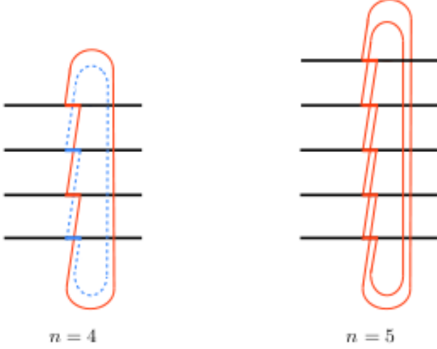
Figure 5. Cut of the Riemann surface defined by \langle \mathcal{T}_n^2(u_2) \bar{\mathcal{T}}_n^2(v_2) \rangle . Left: A typical example for n even ( n = 4 in the figure) showing how the surface decouples in two independent parts, each with half of the sheets. Right: A typical example for n odd ( n = 5 in the figure) showing that the net effect is just a reshuffling of the sheet numeration going from (1, 2, 3, 4, 5) to (1, 3, 5, 2, 4) .
