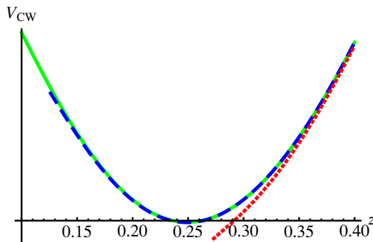
Figure 1. The effective potential normalized in units of \tilde{m}_1^4 y^2 , for F = 2 and y = 10^{-2} (dotted line), 10^{-3} (dashed line) and 10^{-4} (solid line). Each plot ends on the left at the corresponding z_{\min} = z_{\min}(y) . For y > 10^{-3} the would-be minimum would fall into the unstable region of the classical pseudomoduli space and the theory does not have a metastable vacuum. For smaller values of y the minimum exists, and a potential barrier develops against decay toward the supersymmetric runaway vacua at S_0 \rightarrow 0 .
