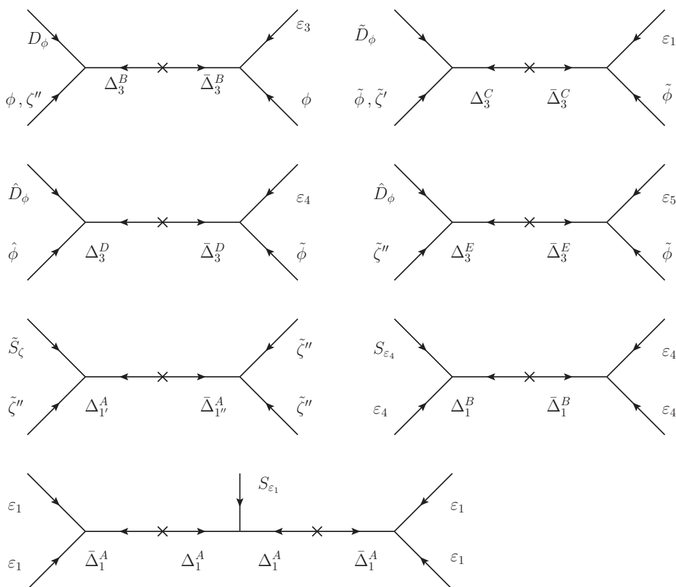
Figure 5. The supergraphs before integrating out the messengers for the flavon sector. We have omitted for simplicity the supergraphs of the higher order corrections in the flavon superpotential.
