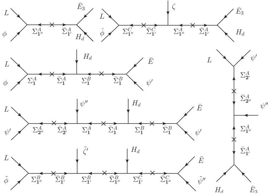
Figure 3. The supergraphs before integrating out the messengers for the charged lepton sector.
