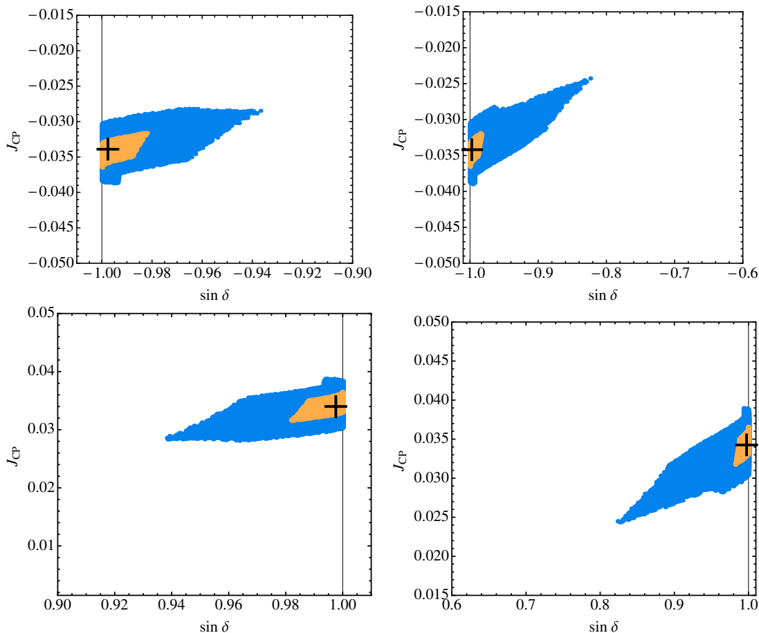
Figure 1. Possible values of \sin \delta and J_{\text{CP}} , obtained by using the 1\sigma (light brown areas) and 2\sigma ranges (blue + light brown areas) of allowed values of the mixing angles \theta_{12} , \theta_{23} and \theta_{13} for NO spectrum (left panels) and IO spectrum (right panels), and for \sin \delta < 0 (upper panels) and \sin \delta > 0 (lower panels). The predictions for the best fit values of \theta_{12} , \theta_{23} and \theta_{13} , corresponding to \delta = 266.02^\circ ( \sin \delta < 0 ) and \delta = 93.98^\circ ( \sin \delta > 0 ), are indicated with crosses. See text for further details.
