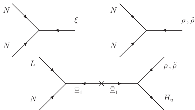
Figure 4. The supergraphs before integrating out the messengers for the neutrino sector.
