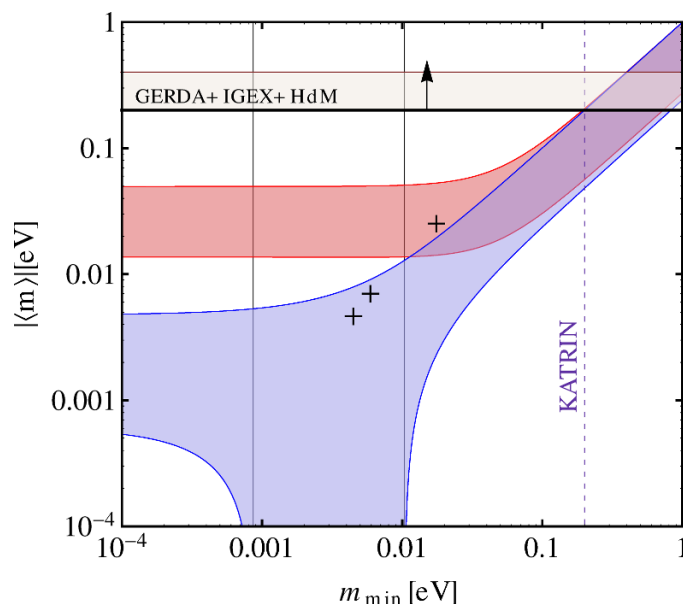
Figure 2. The 3\sigma allowed regions of values of the effective Majorana mass |\langle m \rangle| as functions of the lightest neutrino mass m_{\min} for the NO (blue area) and IO (red area) neutrino mass spectra. The regions are obtained by using the experimentally determined values of the neutrino oscillation parameters (including the 1\sigma uncertainties) quoted in table 1. The black crosses correspond to the predictions of the model constructed in the present article, eqs. (3.78)–(3.80). The horizontal band indicates the upper bound |\langle m \rangle| \sim 0.2 - 0.4 eV obtained using the 90 % C.L. limit on the half-life of ^{76}\text{Ge} reported in [88]. The dotted line represents the prospective upper limit from the \beta -decay experiment KATRIN [89].
