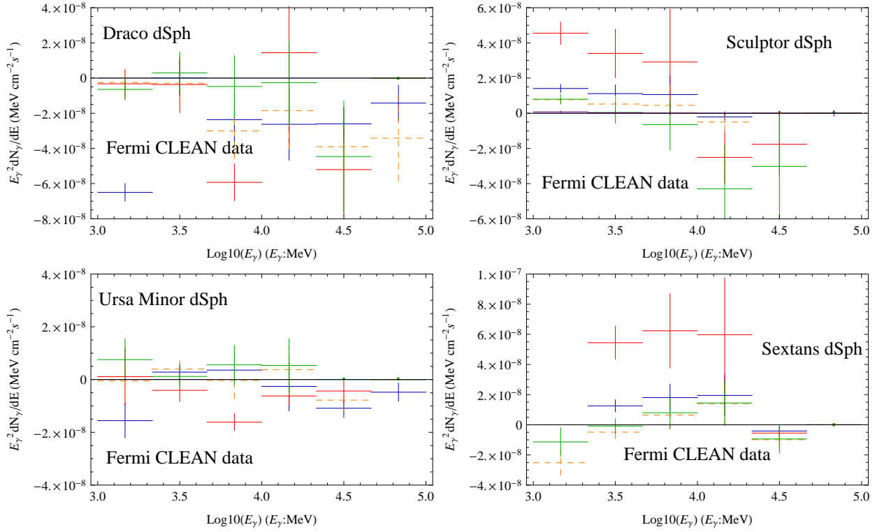
FIG. 5: Excess gamma-ray differential flux for dwarf spheroidal galaxies, using Fermi data “Clean” class. Upper left: Draco, upper right: Sculptor, lower left: Ursa Minor, lower right: Sextans. Dark blue: version 1, red: version 2, dashed orange: version 3, green: version 4.
