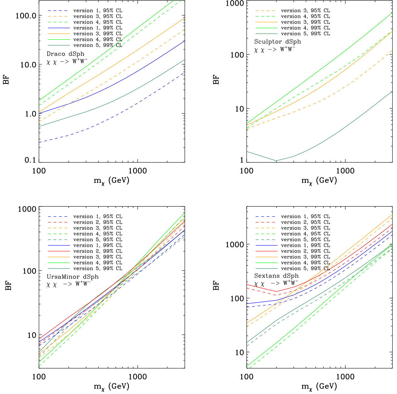
FIG. 10: 95% C.L. and 99% C.L. limits from dwarf spheroidals for versions 1-5 using Fermi CLEAN class data. Upper left: Draco, upper right: Sculptor, lower left: Ursa Minor, lower right: Sextans. For certain targets as Ursa Minor and Sextans, much more robust limits on DM annihilation can be achieved.
