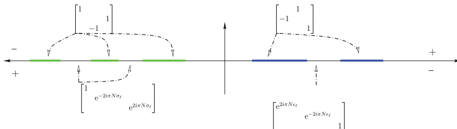
FIG. 6. The RHP for the outer parametrix.
