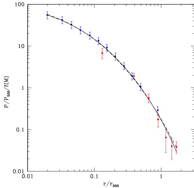
Figure 10. A2204: pressure profiles using XMM-Newton (blue points) and Planck (red points) data (Planck Collaboration et al. 2013a); dashed line is the SM fit with an entropy power law increase while the continuous line is with a flattening of the entropy at r > r_b .
