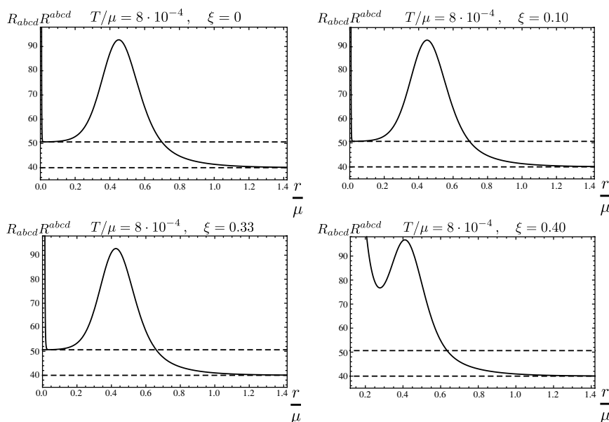
Figure 6. R_{abcd}R^{abcd} as a function of the radial coordinate near the horizon for a low temperature. The horizontal dashed lines indicate the corresponding values of R_{abcd}R^{abcd} for the UV and IR AdS geometries. The stabilization to the IR value, when it happens, holds till very close to the horizon.
