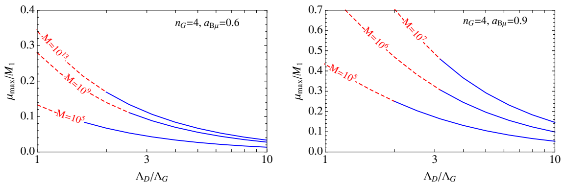
Figure 1. \mu_{\max}/M_1 for a specific choices of parameters: x = 1.2, \xi x = 4.5, \theta = 0.8 (left panel) and x = 0.7, \xi x = 6.7, \theta = 0.7 (right panel). In both cases y \ll 1 is assumed. On the red dashed branch of the curves the coupling \lambda_d gets non perturbative at some point between M and M_{\text{GUT}} .
