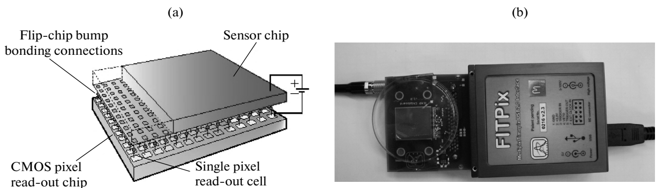
Fig. 8. (a) Structure of a Timepix detector; (b) Timepix pixel detector with USB interface FITPix.
