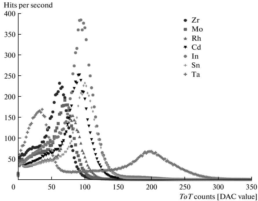
Fig. 12. Summed ToT spectra of different metals used for generalized calibration of Timepix detector.
