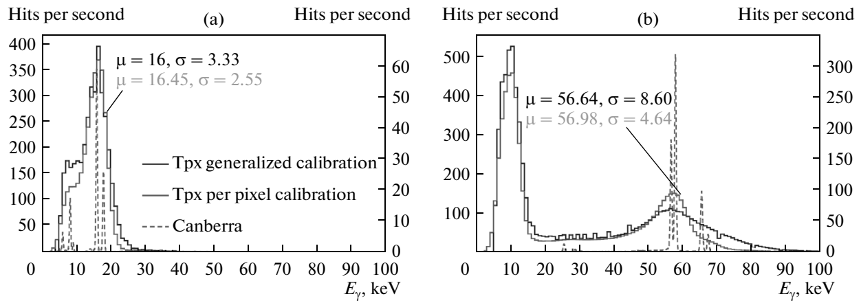
Fig. 17. Spectra of X-ray characteristic emission from Rh (a) and Ta (b) after per-pixel (red) and generalized (blue) calibrations.
