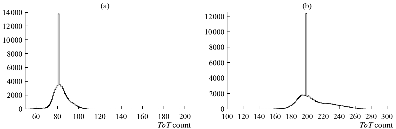
Fig. 15. Distribution of ToT values of the peak position in characteristic spectra of Rh (a) and Ta (b) for all pixels. Spikes in the distributions correspond to the peak positions in the summed spectra (these values are used for “bad” pixels).
