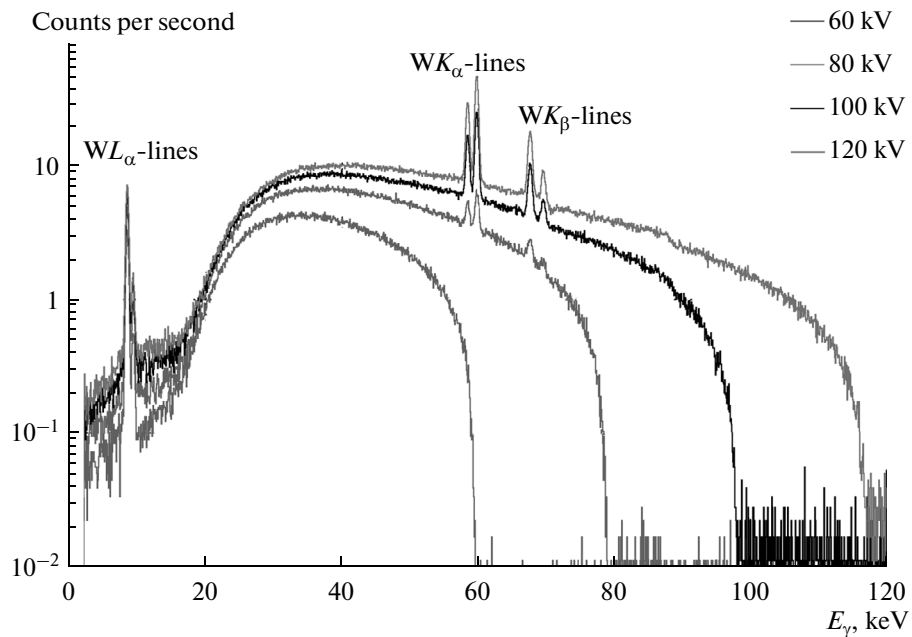
Fig. 3. Emission spectra of SB 120 X-ray tube for different anode voltage.
