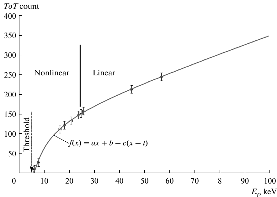
Fig. 10. General shape of the calibration curve ( T ).
