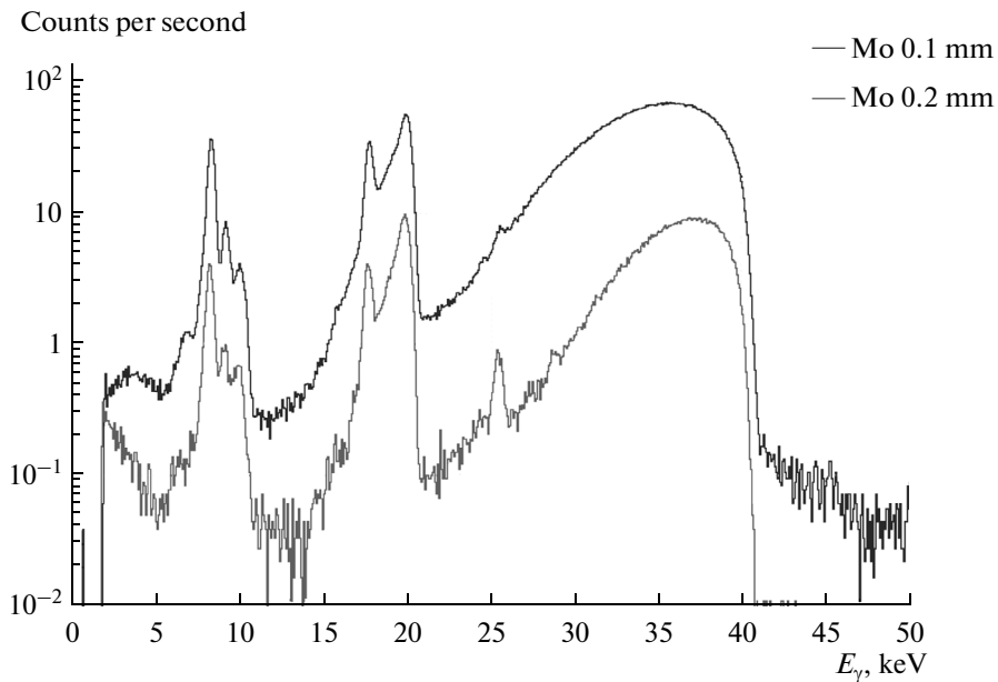
Fig. 7. X-ray spectra in “transmission” geometry from a Mo foil of 0.1 mm (black) and 0.2 mm (grey) thickness.
