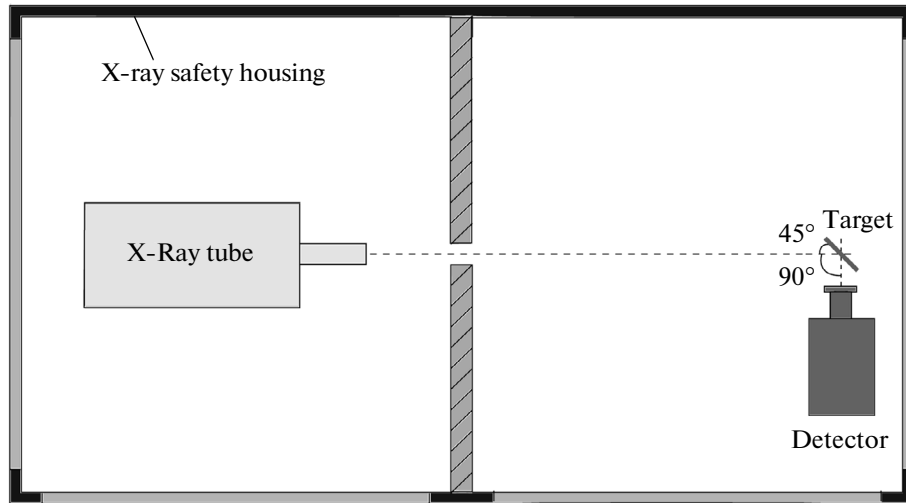
Fig. 4. Layout of the experimental setup for measuring of X-ray spectra in “reflection” geometry.
