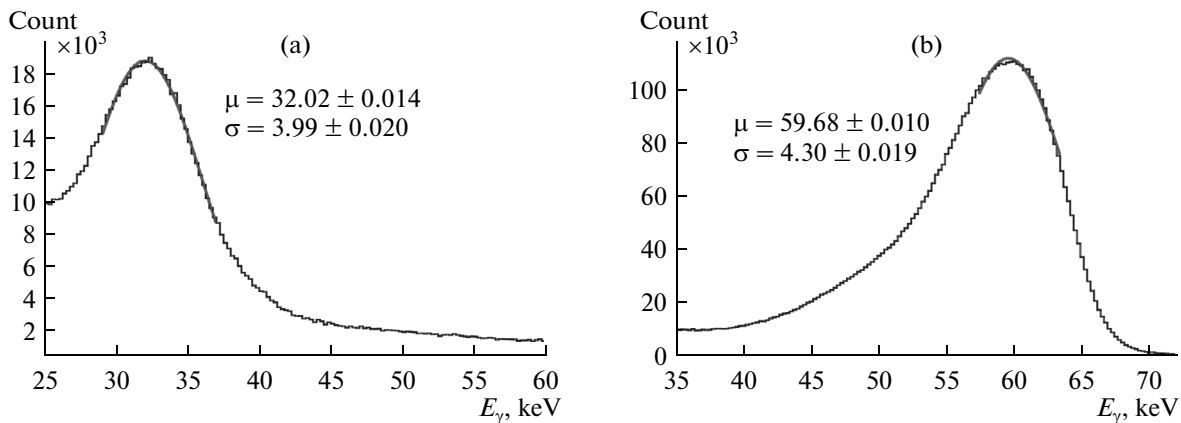
Fig. 19. Spectra of \gamma -radioactive sources measured by the Timepix detector after per-pixel calibration: (a) ^{137}\text{Cs} ( E_\gamma = 32.18 keV); (b) ^{241}\text{Am} ( E_\gamma = 59.54 keV).
