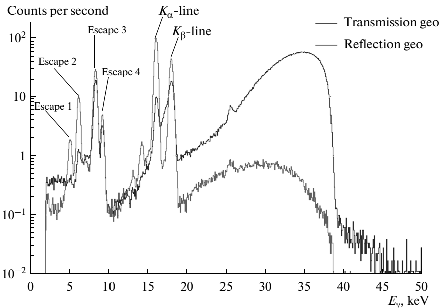
Fig. 5. X-ray spectra from Zr in “transmission” (black line) and “reflection” (grey line) geometries.
