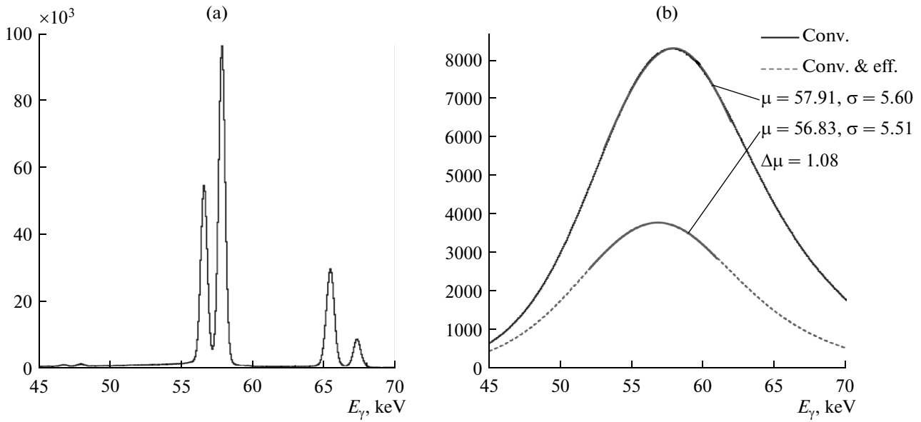
Fig. 11. Spectrum of Ta characteristic X-ray emission in [45, 70] keV range: (a) measured with Canberra detector; (b) modeled by convolution of the Canberra spectrum with the Timepix resolution (solid line) plus absorption efficiency in GaAs (dashed line).
