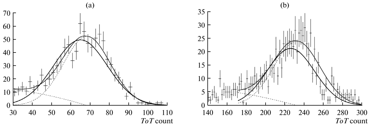
Fig. 14. Fitting with function (3) a single pixel ToT spectra from Rh (a) and Ta (b).
