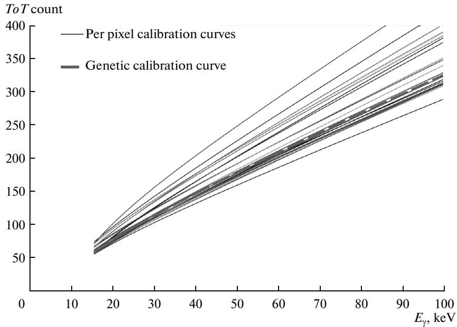
Fig. 16. Per-pixel calibration curves for several pixels (thin lines) and generalized calibration curve (thick dashed line).
