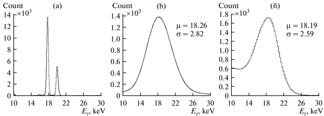
Fig. 18. Spectra of characteristic X-ray emission of Mo in the [10, 30] keV range: (a) measured with Canberra detector; (b) modeled for GaAs Timepix detector; (c) measured with GaAs Timepix detector after per-pixel calibration.
