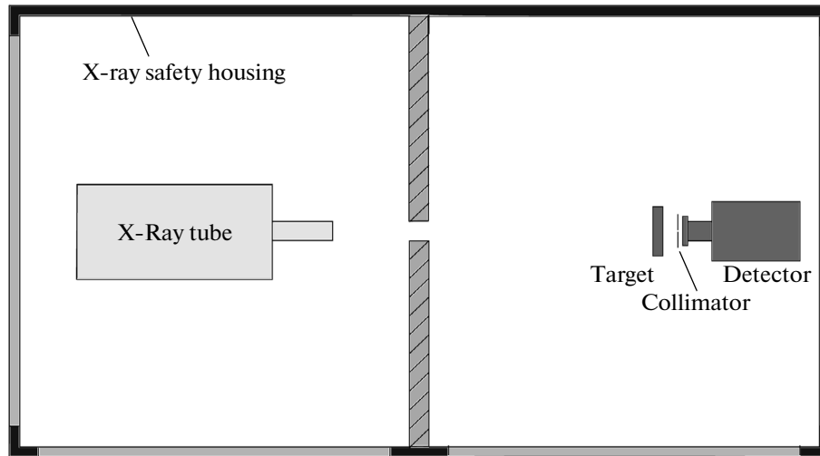
Fig. 1. Layout of the experimental setup for measuring of X-ray spectra.
