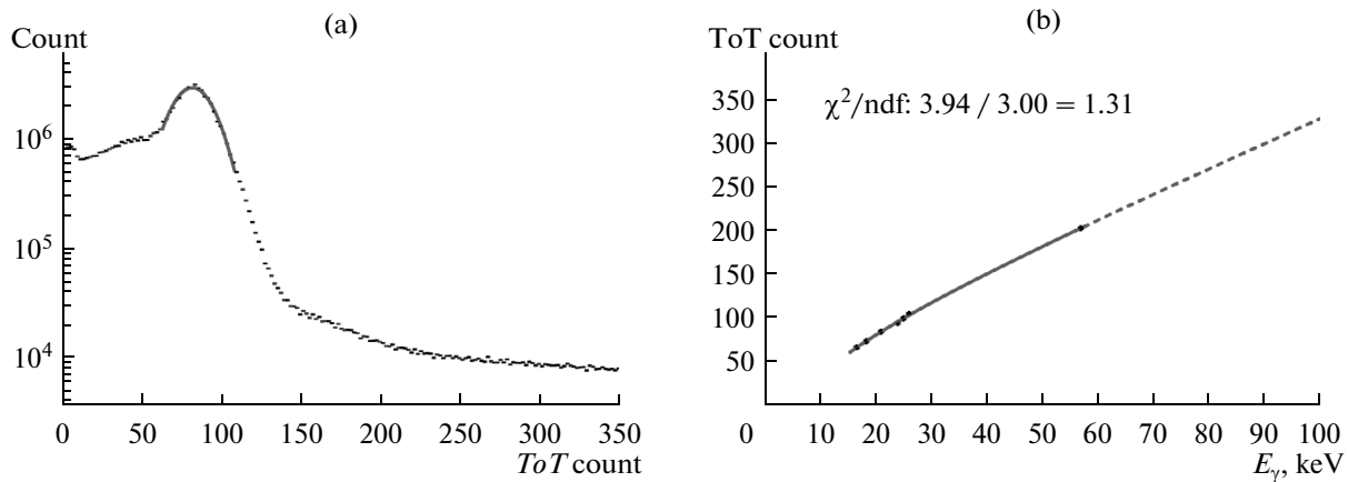
Fig. 13. (a) Gaussian fit of the summed over pixels ToT spectrum of characteristic X-ray emission from Rh; (b) Generalized calibration curve, fitted over seven data points: Zr, Mo, Rh, Cd, In, Sn, Ta.
