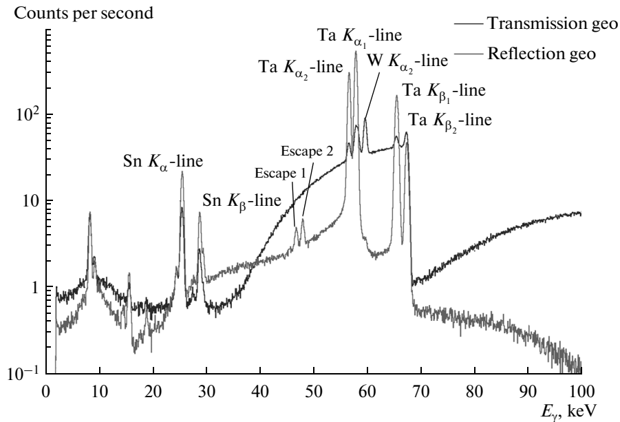
Fig. 6. X-ray spectra from Ta in “transmission” (black line) and “reflection” (grey line) geometries.
