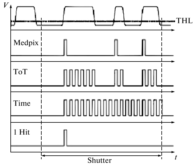
Fig. 9. Modes of operation of Timepix detector. THL —threshold value.
