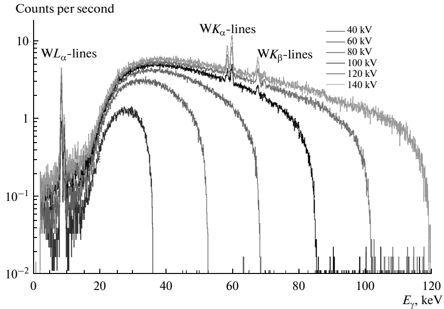
Fig. 2. Emission spectra of RAP-150MN X-ray tube for different anode voltage.
