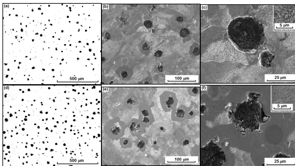
Figure 1. Microstructure of ductile cast iron GJS-600-3U: unmodified (a–c); modified (d–f); as-polished microstructures (a,d); and etched microstructures (b,c,e,f).
