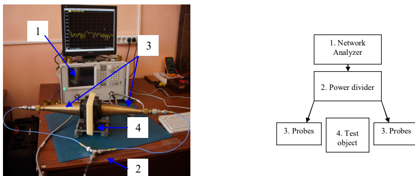
Fig. 2. Breadboard model of the microwave interference microscope.
