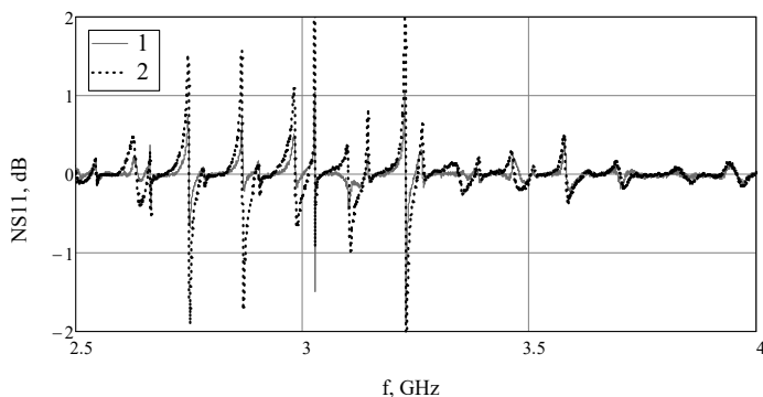
Fig. 5. Frequency dependence of RRC for the laminate 5 mm thick: 1 – with the opening with a diameter of 4 mm, 2 – with the opening with a diameter of 10 mm.
