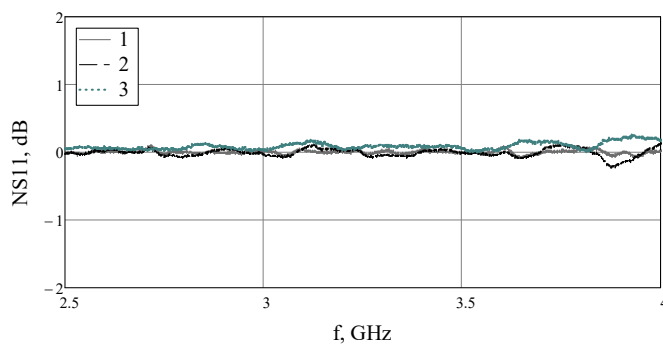
Fig. 6. Frequency dependence of RRC for the laminate 5 mm thick: 1 – the continuous laminate, 2 – with the opening with a diameter of 3 mm, 3 – with the opening with a diameter of 10 mm.
