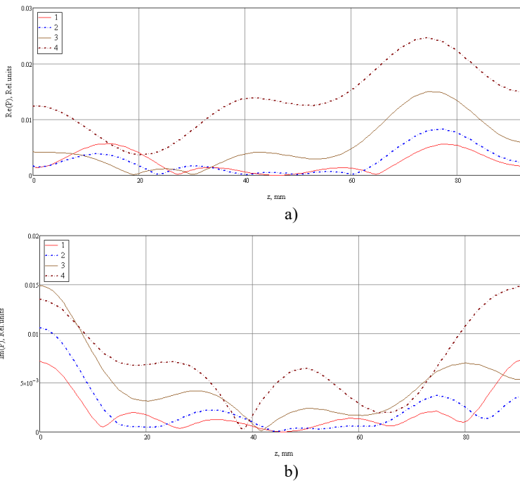
Fig. 1. Distribution of the longitudinal component of complex Poynting's vector in the interval between apertures of two active probes.
