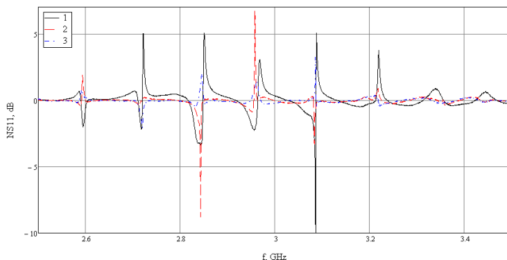
Fig. 4. Frequency dependence of RRC for seeds of three different cultures in the band from 2.5 GHz to 3.5 GHz: 1 – the amaranth, 2 – the impatiens and 3 – soy.
