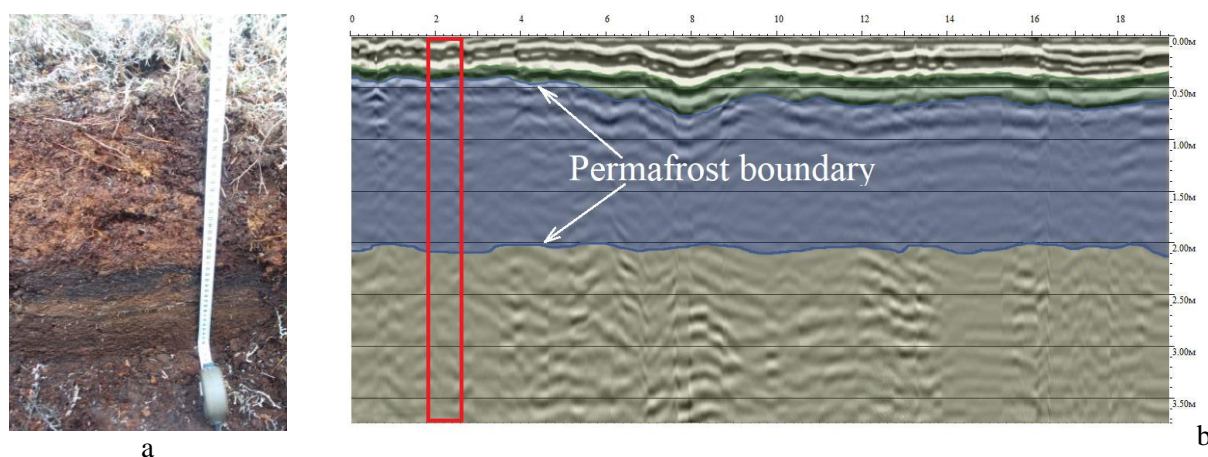
Figure 5. Soil profile 2-17 (a) and radargram 29 (b) of site 1.
