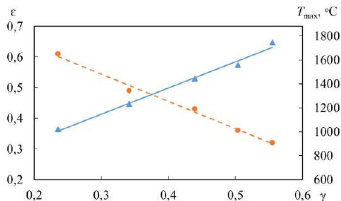
Figure 4. Effective emissivity coefficient of flame ( \bullet ) and maximum temperature ( \blacktriangle ) in the outer flame versus the \gamma parameter, T_v = 250^\circ\text{C}
