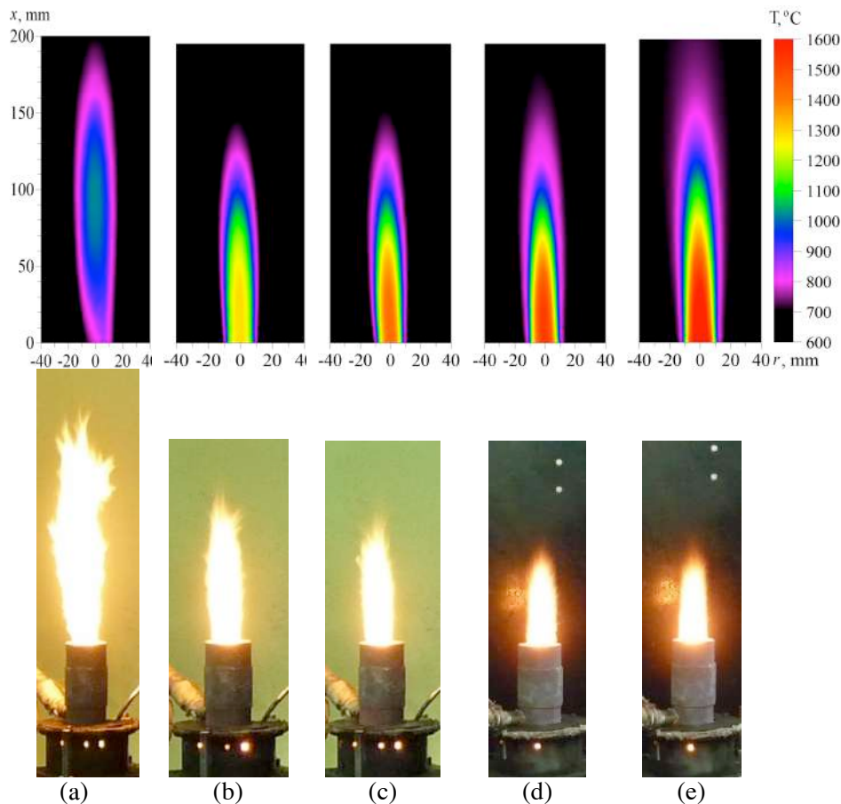
Figure 2. Thermograms of flame and the photographs for different steam flow rates (at a constant temperature steam T_v \sim 250 °C: \gamma = 0.24 (a), \gamma = 0.34 (b), \gamma = 0.44 (c), \gamma = 0.50 (d), \gamma = 0.56 (e), and a steam pressure in the range of 8±2 atm, respectively)
