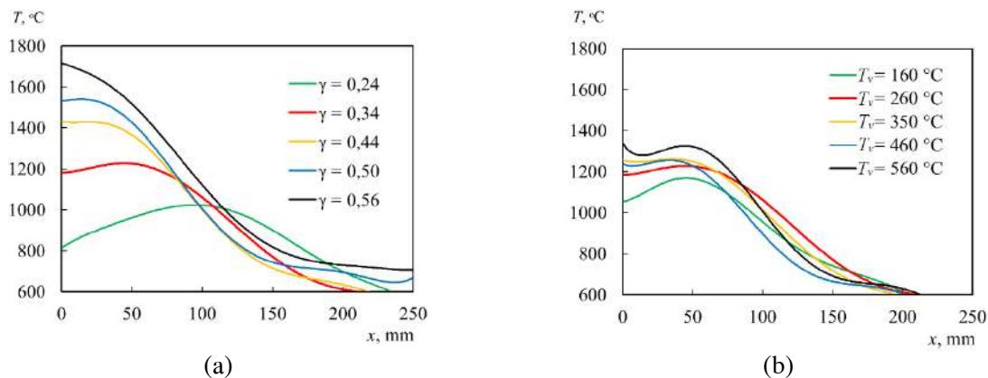
Figure 3. Distribution of the time-average temperature in the outer flame along the vertical center line of the flame for different mode parameters: (a) the steam flow rate is varied, T_v = 250^\circ\text{C} ; (b) the steam temperature is varied, \gamma = 0.34 , the steam pressure is 4 atm
