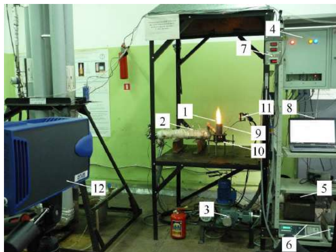
Figure 1. Combustion stand for the study of liquid hydrocarbon combustion with steam gasification: 1 is the burner device, 2 is the electric steam generator, 3 is the plunger metering pump, 4 is the automatic steam generator control system, 5 is the fuel supply system, 6 is the electronic balance, 7 is the indicators of control and measurement instruments, 8 is the computer, 9 is the gas-generation chamber of the furnace unit, 10 is the combustion chamber of the furnace unit, 11 is the fuel pipe, 12 is the thermal imager
