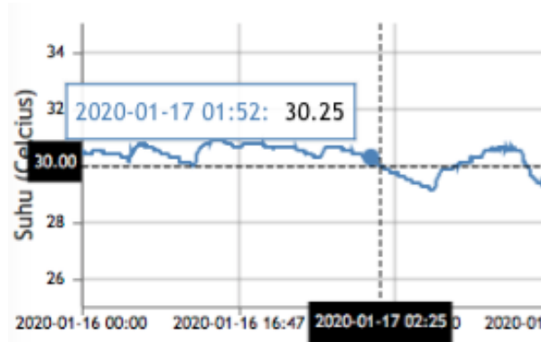
Figure 6: Temperature fluctuation at set point 30 °C
