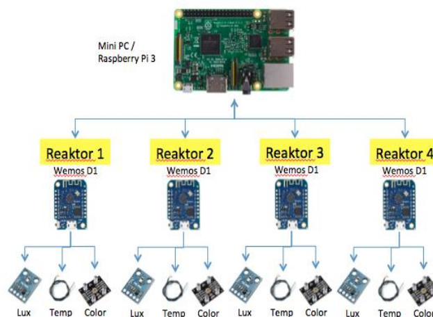
Figure 5: Sensor configuration of each reactor
