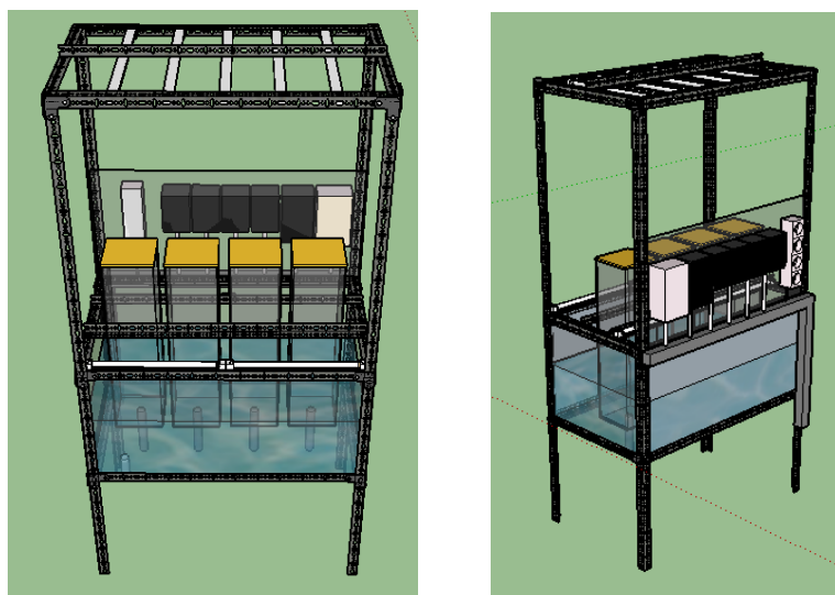
Figure 3: Fotobioreactor design (a) Front (b) Rear
