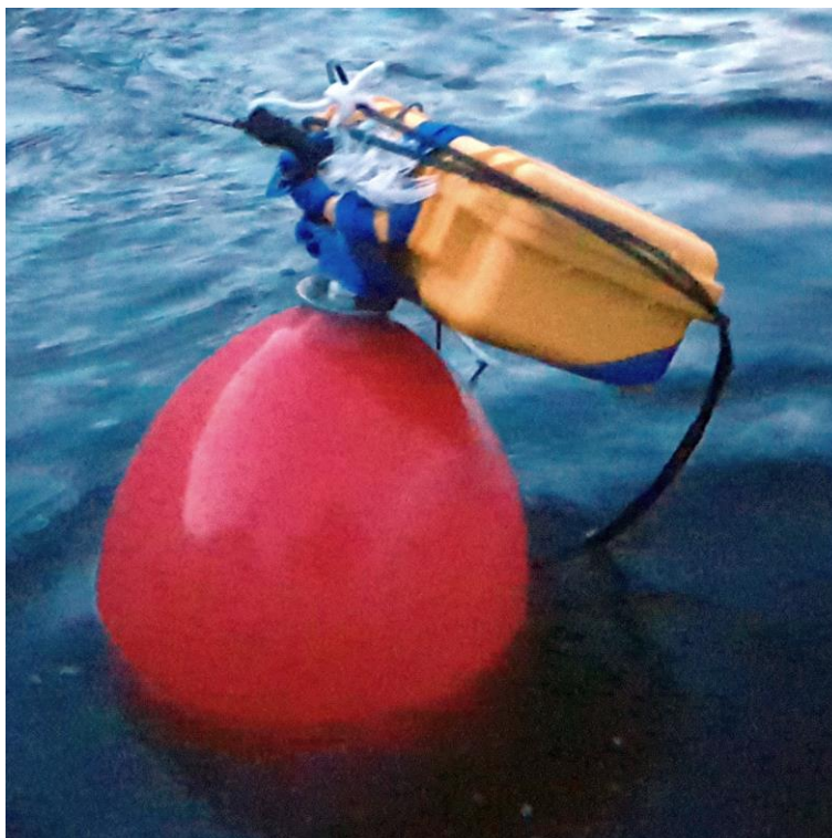
Figure 3. Direct deployment of logger and temperature cable from a boating buoy.
