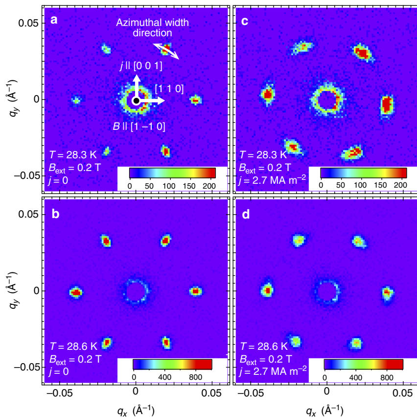
Fig. 2 Small angle neutron scattering (SANS) data for investigating the peak broadening of the skyrmion reflection. a–d SANS measured at B_{\text{ext}} = 0.2 T. The skyrmion reflections were measured at T = 28.3 K ( 28.6 K) under j = 0 ( 2.7 \text{ MA m}^{-2} ), respectively. All data were measured for 10 min. When the intensities of the six skyrmion reflections are not equivalent, the sample is slightly misoriented away from the Bragg position. The azimuthal width direction is indicated by the arrow in panel a . q_x and q_y stand for the reciprocal lattice space directions
