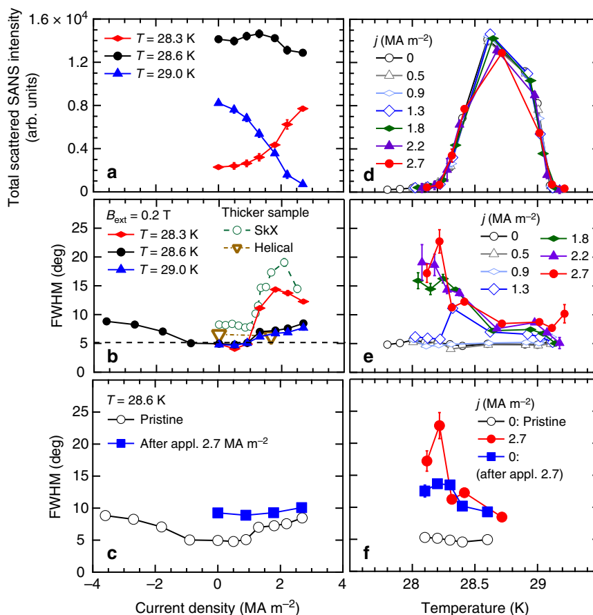
Fig. 3 Current-density and temperature dependences of the skyrmion reflections for investigating the peak broadening of the skyrmion reflection. a–c , Current-density dependences of the total scattered small angle neutron scattering (SANS) intensity ( a ) and the azimuthal spot widths ( b and c ) of the skyrmion reflections measured at three temperatures. Here, we use 1\sigma standard deviation as error bar. The temperature used in a–c is the sensor temperature, and therefore not the true temperature estimated from the ordering temperature of the helical phase. Thus, the increase (decrease) of the intensity at T = 28.3 K (29.0 K and 28.6 K) under the high electric current is due to sample heating. For the measurement of the negative current density, we reset the peak broadening of the skyrmion reflection at zero current density once by heating the sample above the phase transition temperature. In a and c–f , data are measured at B_{\text{ext}} = 0.2 T. In b the azimuthal width of the skyrmion ( B_{\text{ext}} = 0.2 T) and helical ( B_{\text{ext}} = 0 ) reflections at T = 28.6 K measured by the thicker sample are also shown. d–f Temperature dependences of the total scattered SANS intensity ( d ) and azimuthal widths ( e , f ) of the skyrmion reflections at each current density. In c and f additionally, the dependence of the width after applying j = 2.7 MA m ^{-2} is shown. The broadening of the skyrmion reflection persisted for more than one hour after the applied current density was removed
