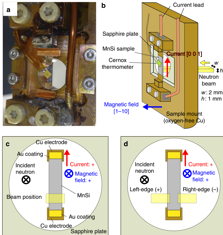
Fig. 1 Experimental setting of small angle neutron scattering (SANS) with keeping any thermal gradient as small as experimentally achievable. a, b Photograph ( a ) and schematic drawing ( b ) of the MnSi sample and sample mount for the NG7 experiment. The incident neutron beam was shaped to be 2.0 mm (width) \times 1.0 mm (height) by an aperture. c, d Schematic illustration of the beam illumination area for investigating the peak broadening ( c ) and counter-rotating behavior at the sample edges ( d ) of the skyrmion-lattice peaks
