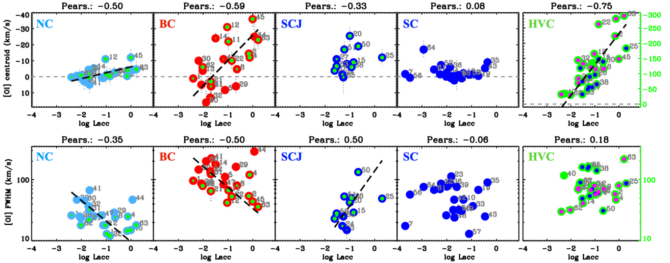
Figure 7. Correlations between [O] properties and accretion luminosity. A similar figure displaying correlations with the veiling is included in the Appendix (Figure 24). Linear fits are shown as black dashed lines, their best-fit parameters reported in Table 7. Color-coding as in Figure 3. Note the different y axis range for the HVC centroids, in the top right plot.
