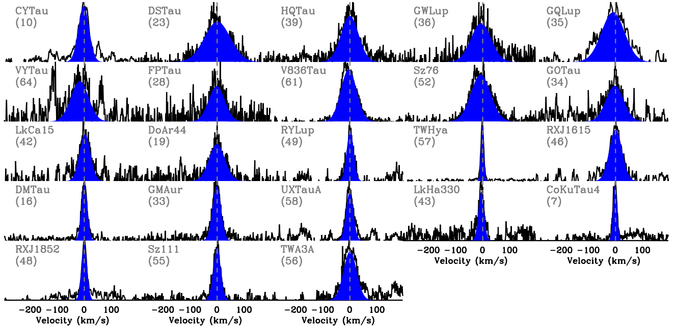
Figure 18. [OI] line profiles and velocity components for “SC” objects, ordered by n_{13-31} index (Figure 10). Sz111 and TWA3A do not have n_{13-31} measurements, and are put at the end. The two symmetric features at the sides of [OI] emission in VYTau are considered spurious (see Figure 21).
