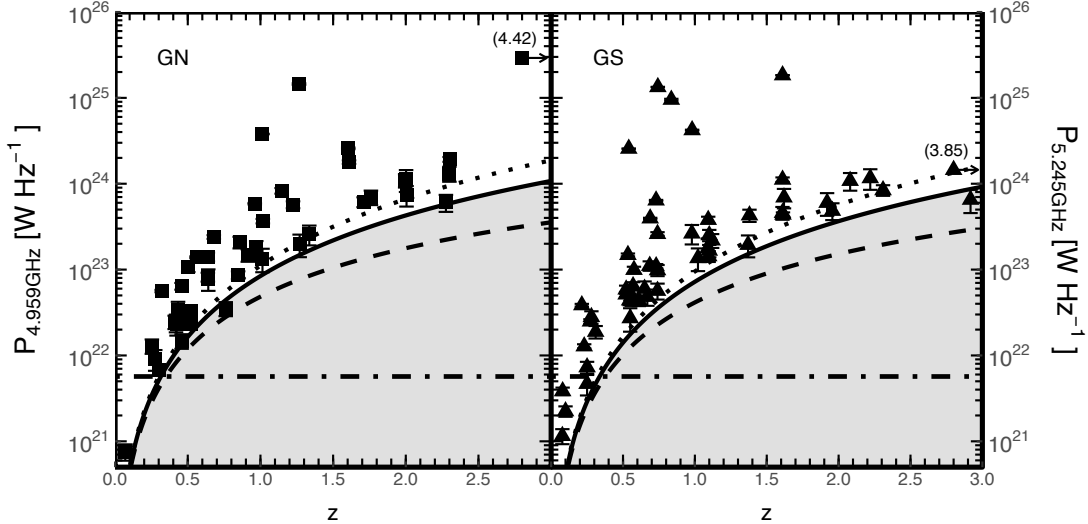
Figure 3. Rest-frame 5 GHz radio power as a function of redshift. Only the radio sources with a spectroscopic redshift are shown. The 5\sigma detection limits are shown for radio spectral index of \alpha = 0 (dashed line), 0.8 (solid line), and 1.2 (dotted line), where S \propto \nu^{-\alpha} . The horizontal dot-dashed line at P_{5\text{GHz}} = 5.7 \times 10^{21} \text{ W Hz}^{-1} corresponds to a luminous infrared galaxy (LIRG) with a SFR = 10 M_{\odot} \text{ yr}^{-1} . Sources with redshift beyond 3 are marked with arrows and their redshifts are written inside the parentheses.
