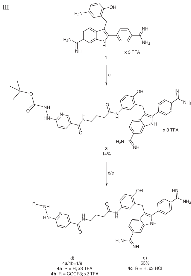
Scheme 2 The synthesis of the new HYNIC-DAPI conjugate. (c) 2 , CDI, DMF, room temperature, 1 day; (d) TFA, room temperature, 1 day; (e) 4 M HCl, room temperature, 1 h.
