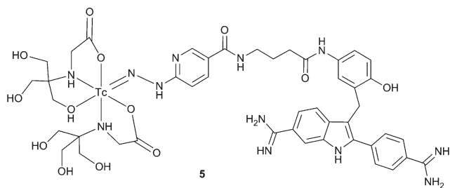
Fig. 1 Proposed structure of ^{99m}\text{Tc}(\text{tricine})_n\text{HYNIC-DAPI} with HYNIC as a monodentate ligand.
