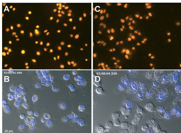
Fig. 3 Distribution characteristics of DAPI (A, B) in comparison with unlabelled HYNIC-DAPI (C, D) in FRTL5 cells. The fluorescence images (A and C) were recorded using the DAPI filter of an Axioskop 40 microscope (Zeiss) and show the cell nuclei of fixed cells. The live cell images (B and D) show the correlation of differential interference contrast (DIC) technique and DAPI filter (Axio Observer Z.1 microscope from Zeiss).
