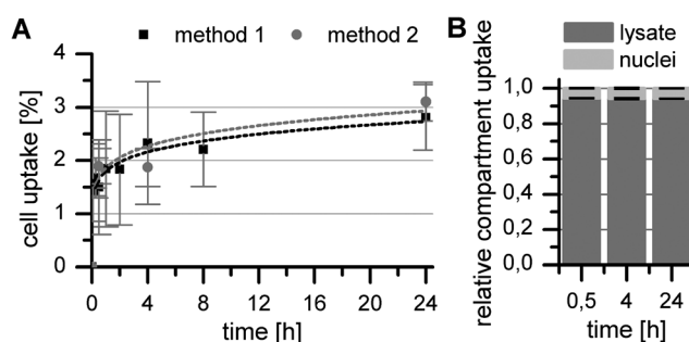
Fig. 5 (A) Internalisation characteristics of ^{99m}\text{Tc} -HYNIC-DAPI. Method 1 (—): cells detached with sodium hydroxide; method 2 (—): cells treated with nuclei isolation kit. (B) Relative distribution pattern of ^{99m}\text{Tc} -HYNIC-DAPI from compartmental analysis (method 2) based on the cell uptake.
