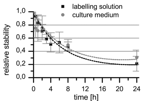
Fig. 6 Stability of ^{99m}\text{Tc} -HYNIC-DAPI derivatives in labelling solution (pH 5, room temperature) and culture medium (pH 7.2, 37 °C) over incubation times of 24 h.
