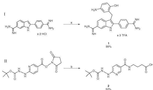
Scheme 1 Syntheses of compounds 1 and 2 . (a) 1 . Koshland's reagent, water, acetone, room temperature, 1 day; 2 . formic acid, 10% Pd/C, TFA, water, 100 °C, 1 day; (b) GABA, Hünig's base, DMF, room temperature, 1 day.
