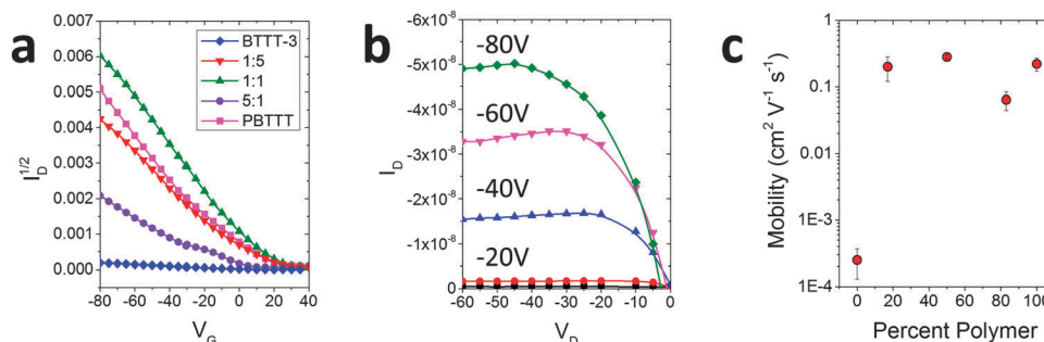
Fig. 6 Characteristics for polymer/oligomer blend OFETs (a) Square root of transfer curves. V_{DS} = -60 V (b) characteristic output curve for the 5:1 blend. Gate voltages are noted in the figure. (c) Graph of mobilities vs. percent of polymer in blend composition.
