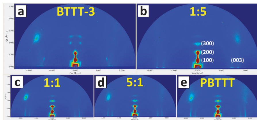
Fig. 3 Grazing-incidence wide-angle X-ray scattering (GIWAXS) diffractograms of (a) 100% BTTT-3, (b) 87% BTTT-3/13% PBTTT, (c) 50% BTTT-3/50% PBTTT, (d) 13% BTTT-3/87% PBTTT, and (e) 100% PBTTT thin films. The Q_{xy} value of the peaks for the pure BTTT-3 film corresponds to 3 \text{ nm} , indicating that the oligomer is fully extended in its crystal packing. In the films that contain a nominal amount of polymer, the diffraction is virtually identical to the pure polymer film.
