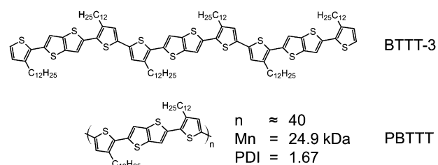
Fig. 1 Molecular structures of the oligomer, BTTT-3, and polymer, PBTTT, used in this study.
