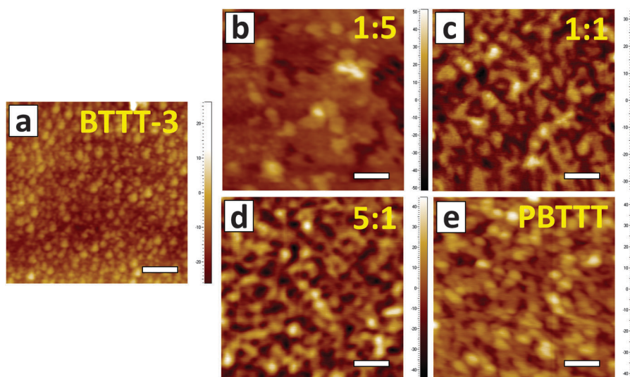
Fig. 2 Atomic force micrographs: surface height of (a) 100% BTTT-3, (b) 87% BTTT-3/13% PBTTT, (c) 50% BTTT-3/50% PBTTT, (d) 13% BTTT-3/87% PBTTT, and (e) 100% PBTTT thin films. Scale bar is 200 nm. Vertical scale is in \text{\AA} .
