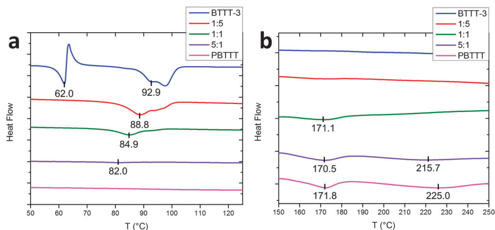
Fig. 5 Differential scanning calorimetry traces for the side chain and backbone melting regions of (a) BTTT-3 and (b) PBTTT (endo down). Note the absence of the BTTT-3 side chain melting at 62.0 °C for all blends that contain PBTTT. The depressed melting points for the BTTT-3 and PBTTT backbones from 92.9 °C to 82.0 °C and 225.0 °C to 215.7 °C, respectively, indicated that the crystallites were less pure.
