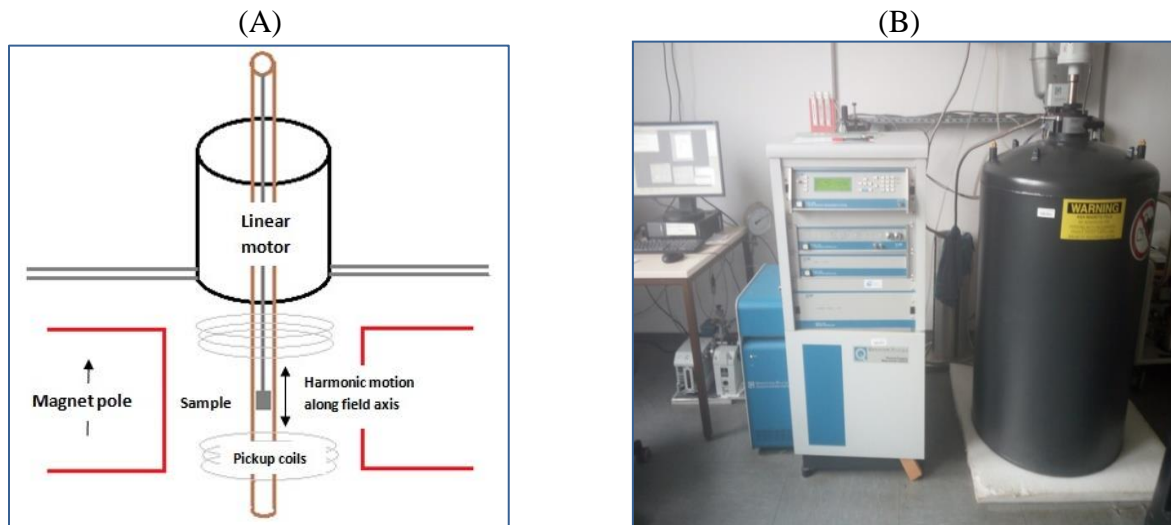
Figure 3.8: (A) VSM option of the PPMS setup (B) a photo of the PPMS at JCMS-2.
