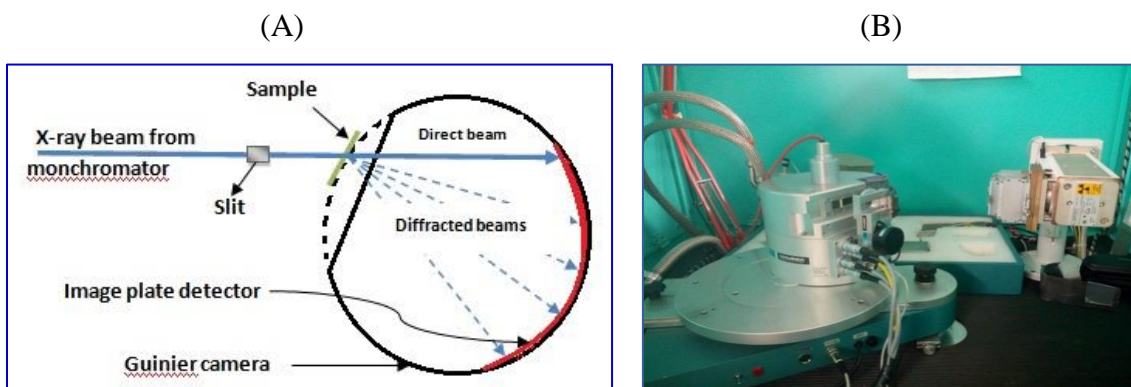
Figure 3.5: (A) Schematic representation of a powder diffractometer with transmission geometry (B) A photo of the diffractometer used in this work.
