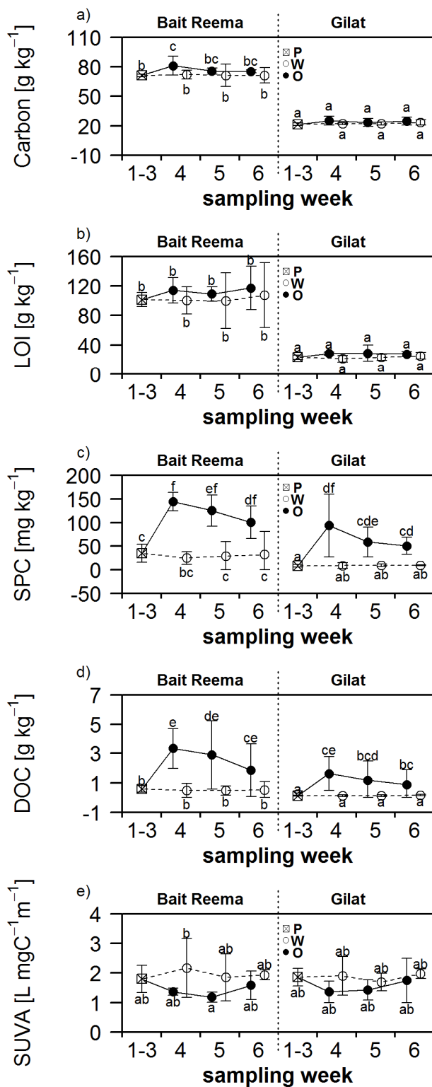
Figure 4. Evolution of soil carbon content, loss on ignition (LOI), soluble phenolic content (SPC), dissolved organic carbon (DOC) and specific UV-adsorption at 254 nm (SUVA 254 nm ) following amendment with OMW and water during six weeks of sampling in Bait Reema and Gilat. P, data before the application (were averaged after finding no statistical differences between three sampling weeks); W, water application; O, OMW application. Mean values followed by the same letter are not statistically different. Error bars show ±95 % confidence intervals.
