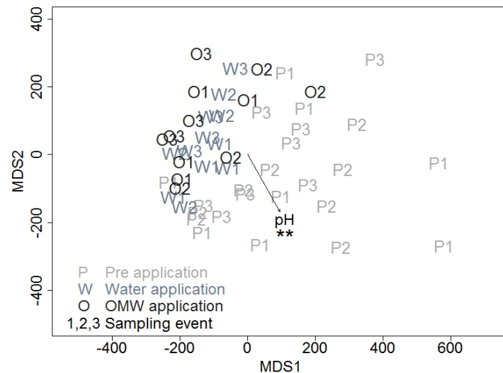
Figure 5. Non-metric multidimensional scaling based on the Oribatida and Collembola community in Bait Reema. Arrow of the explanatory variable pH points to the direction of the increasing gradient, the length is proportional to the correlation between the variable and the ordination. Ordinations are based on Bray-Curtis dissimilarity after Wisconsin double standardization of the community matrix. Asterisks code significant relationships (** p < 0.01 ) between community composition and environmental parameters. P, pre application; W, water application; O, OMW application at the 1st, 2nd and 3rd sampling interval.
