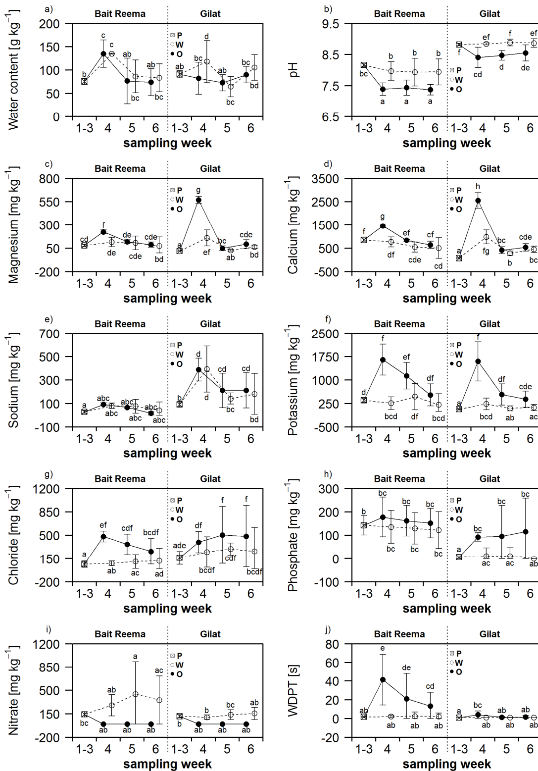
Figure 3. Evolution of water content, pH, concentration of nutrient cations as well as anions and chloride and wettability following amendment with OMW and water during six weeks of sampling in Bait Reema and Gilat. P, data before the application (were averaged after finding no statistical differences between three sampling weeks); W, water application; O, OMW application. Mean values followed by the same letter are not statistically different. Error bars show \pm 95\% confidence intervals.
