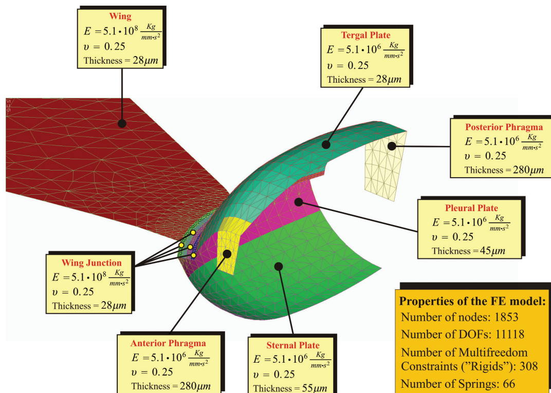
Figure 10. Finite Element Model: Material and Structural Data.
