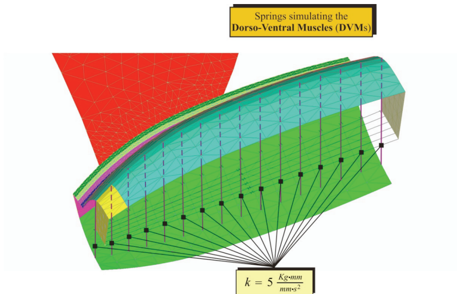
Figure 9. Simulation of the Dorso-Ventral Muscles (DVMs).
