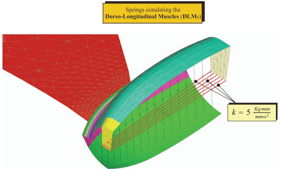
Figure 8. Simulation of the Dorso-Longitudinal Muscles (DLMs).
