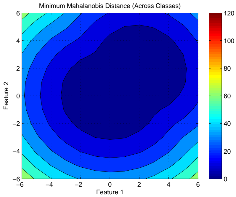
Figure 5.7 Mahalanobis Distance for Discrete Points.
