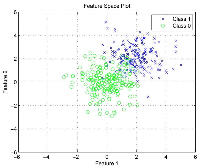
Figure 5.1 Two-Class Feature Space Plot (200 Observations Each).
