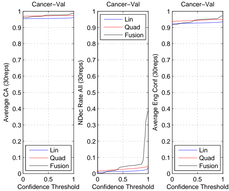
Figure 7.8 Cancer-Three Performance Parameters vs. Confidence Threshold-Validation Set.
