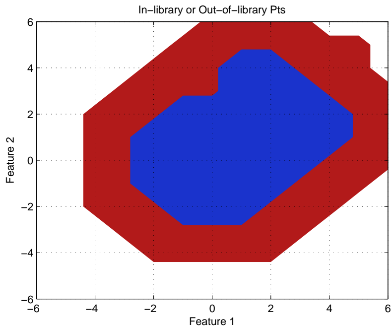
Figure 5.9 GRNN Feature Map using Two Thresholds.
