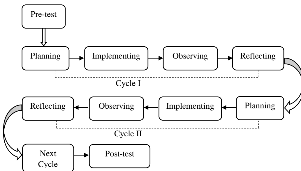
Figure 1: Research Design
