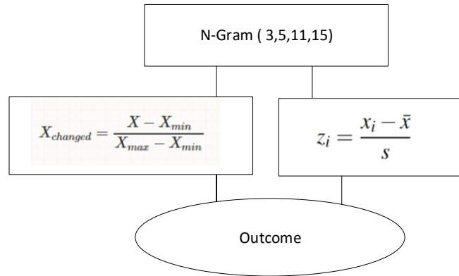
Fig. 1. Normalization process
