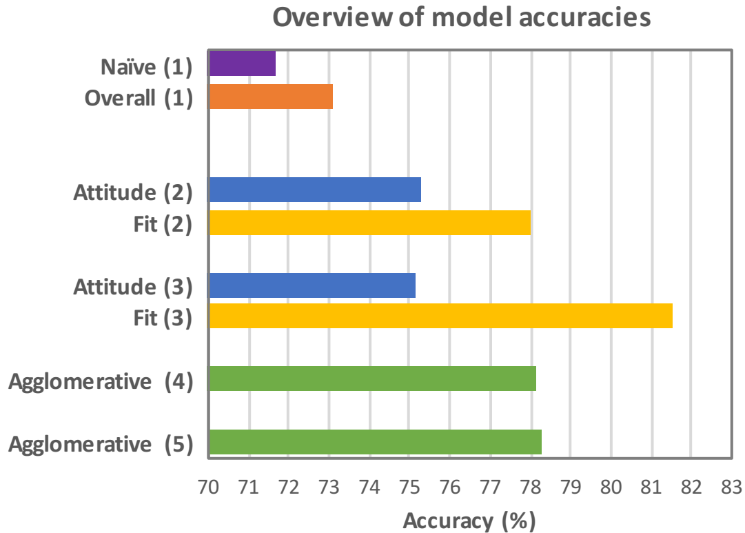
Figure 4.7: Accuracy of our clustering approaches
