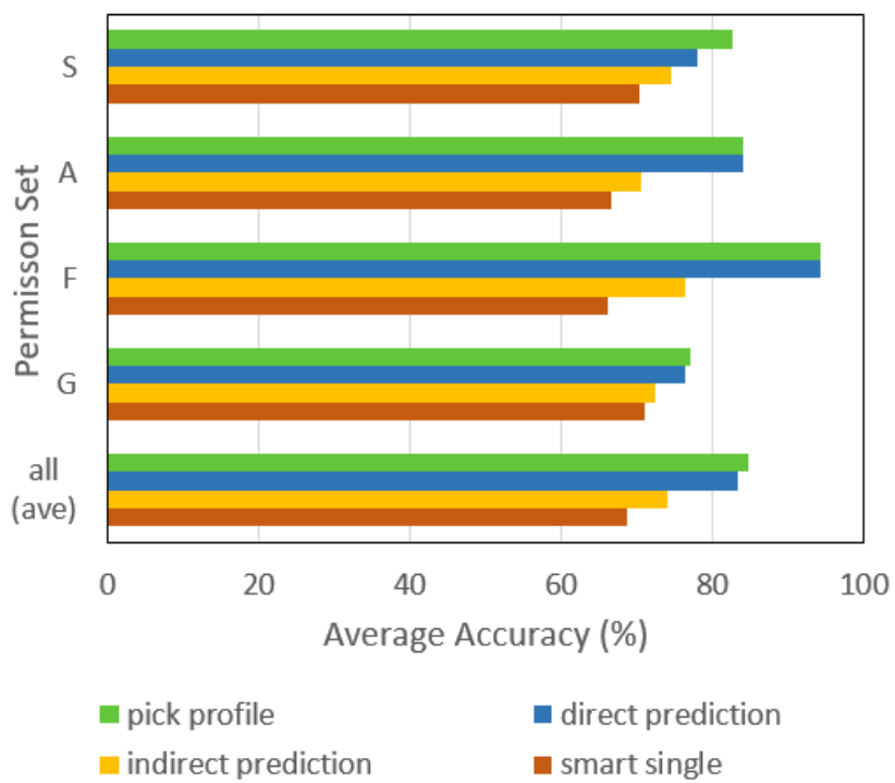
Figure 6.17: Average accuracies of the recommender strategies on the holdout 30 users.
