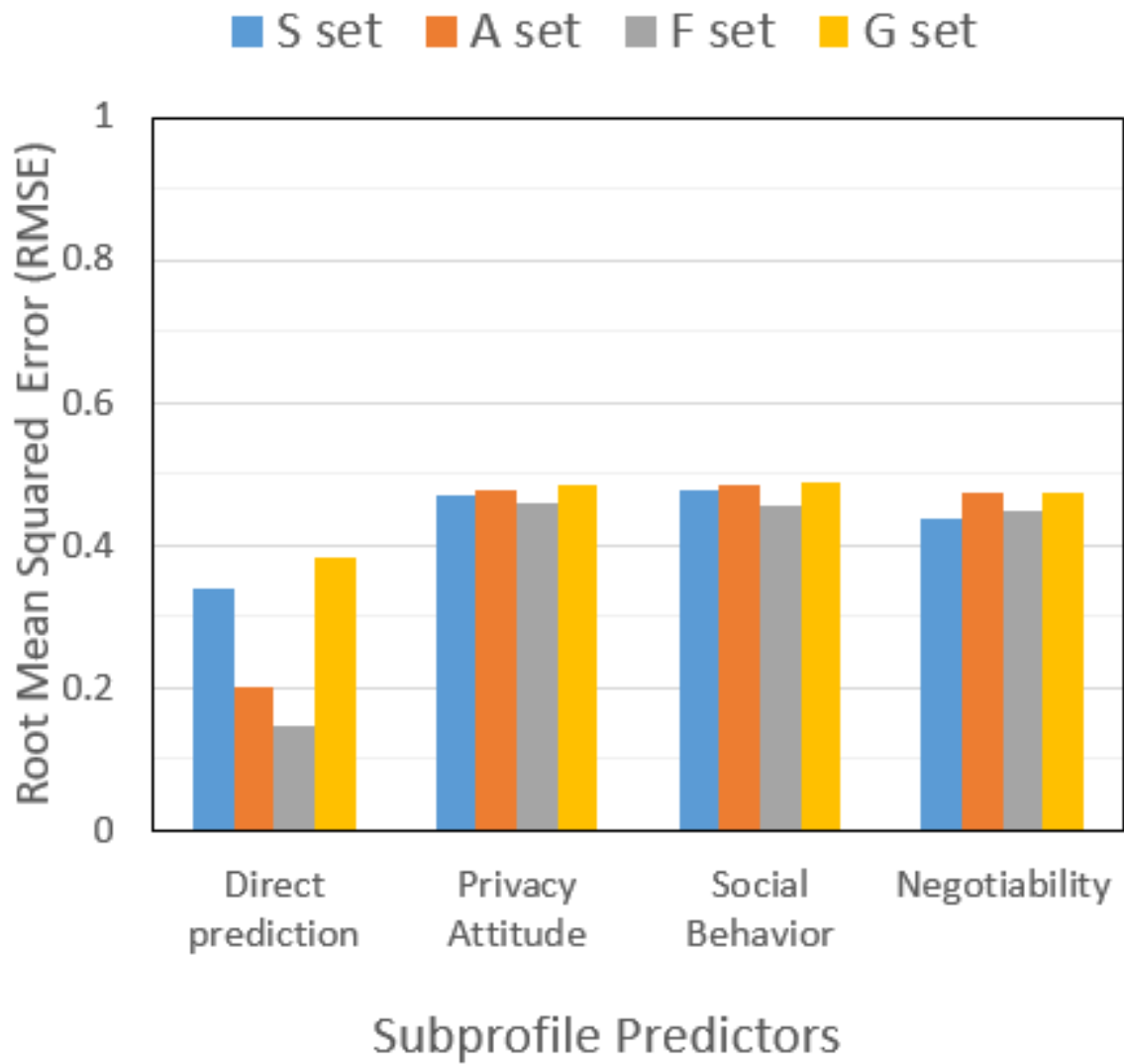
Figure 6.11: Tree evaluation. Root mean square error for each J48 tree algorithm.
