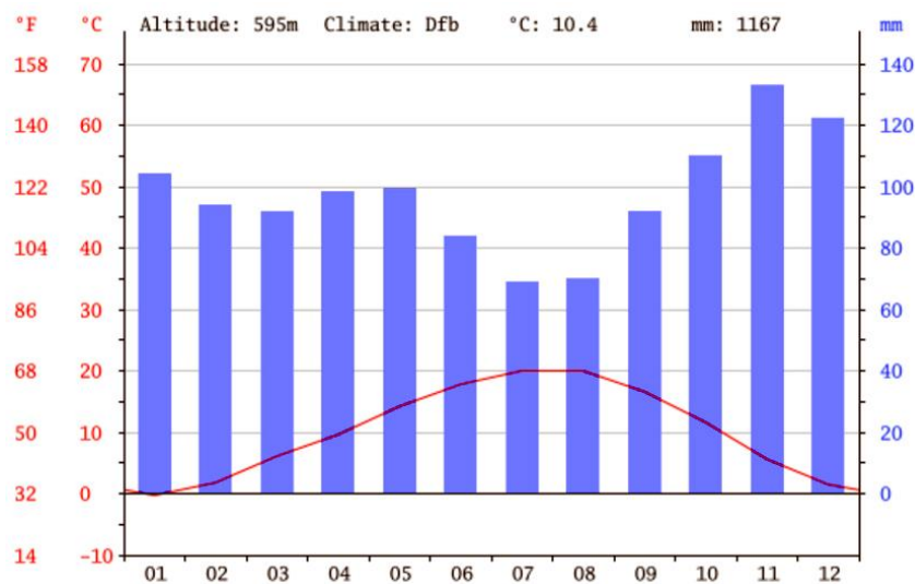
Figure 2. Climate graph
