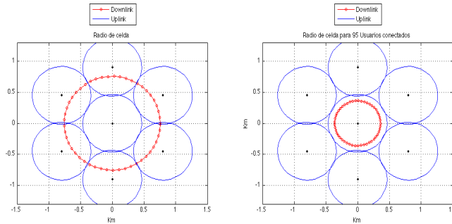
Figure 8: Coverage variation for low and high traffic load.
