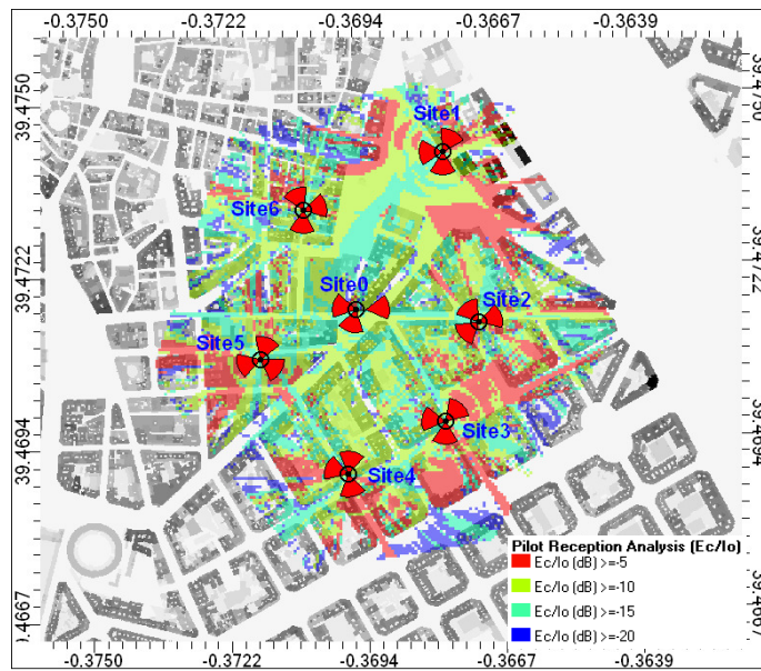
Figure 12: RSCP CPICH Static Power
