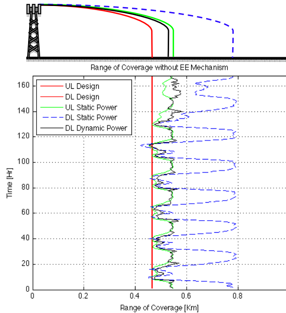
Figure 10: Radio Coverage Adjustment by the forecasted traffic.
