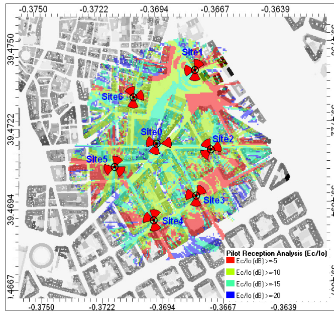
Figure 13: RSCP CPICH Dynamic Power
