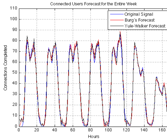
Figure 4: Forecasting applying auto-regressive models
