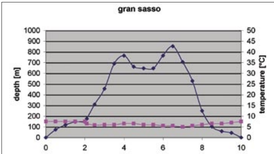
Fig. 4: Depth profile and rock temperatures in the Gran Sasso tunnel.
