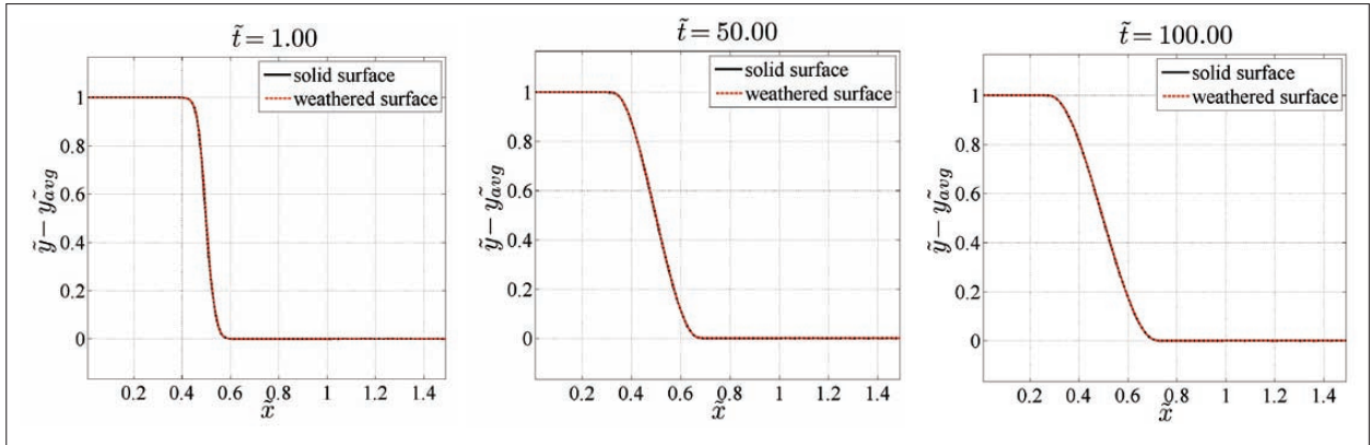
Fig. 5: Evolution of slope: Dominant chemical weathering (example 3).
