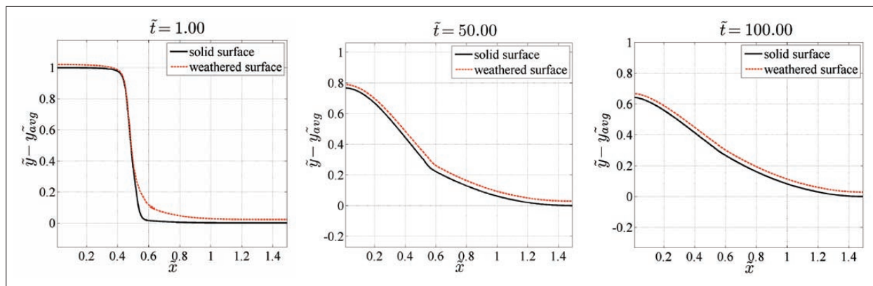
Fig. 3: Evolution of slope: Dominant mechanical weathering (example 1).
