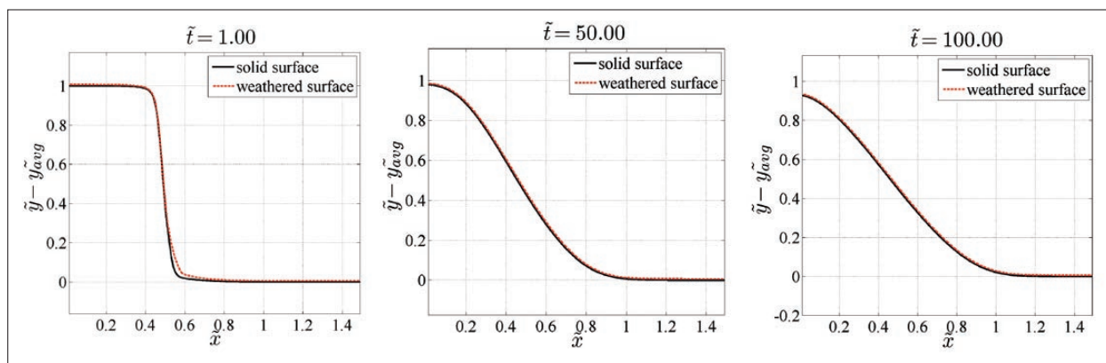
Fig. 4: Evolution of slope: Balanced mechanical and chemical weathering (example 2).
