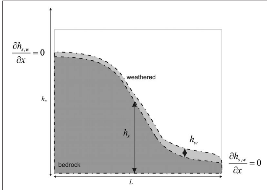
Fig. 2: Model setup.
