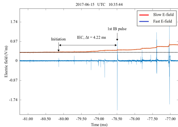
Fig. 2. An Initial Electric Field Change (IEC) (Physic sign convention) and the first Initial Breakdown (IB) pulse for a Negative Cloud-to-Ground (–CG) flash (within reversal distance) captured by wideband fast and slow antenna systems in Malacca at 10:35:44 UTC on June 15th, 2017
