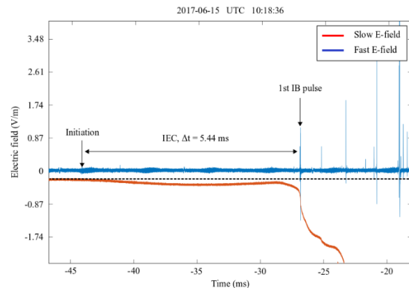
Fig. 3. An IEC (Physic sign convention) preceded the first IB pulse for an Intra Cloud (IC) flash (within reversal distance) captured by wideband fast and slow antenna systems in Malacca at 10:18:36 UTC on June 15th, 2017
