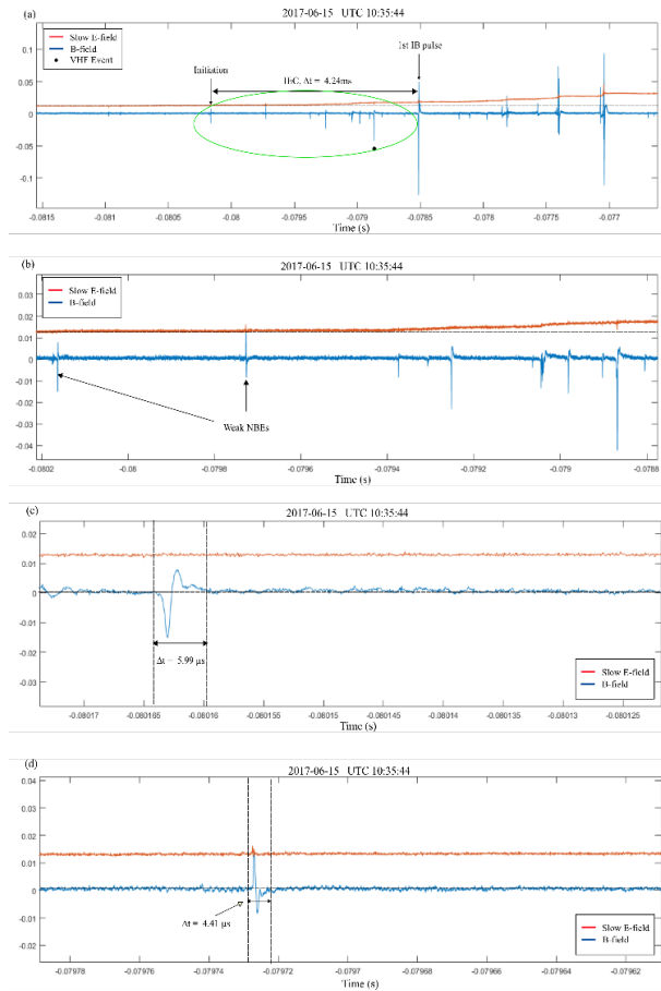
Fig. 6. An IEC for -CG flash. (a) Show the IEC for -CG flash from tropical storm on June 15th, 2017 at 10:35:44 UTC. The green circle is to mention about the small pulses. (b) This figure shows the pulses inside green circle from (a) and some of small pulses got positive and negative polarity. (c) Example of small pulses with average pulse duration of 5.99 \mu s for negative polarity. (d) Example of small pulses with average pulse duration of 4.41 \mu s for positive polarity
