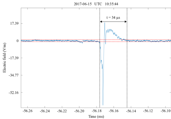
Fig. 1. A classical Initial Breakdown (IB) pulse for a –CG flash captured with wideband fast antenna system on June 15th, 2017 at 10:35:44 UTC (Physics sign convention)
