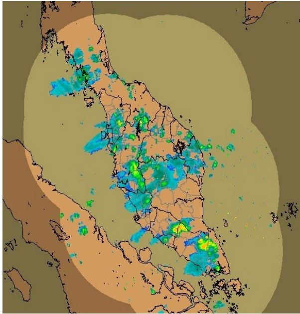
Fig. 4. CAPPI radar data at 2 km altitude for Peninsular Malaysia
