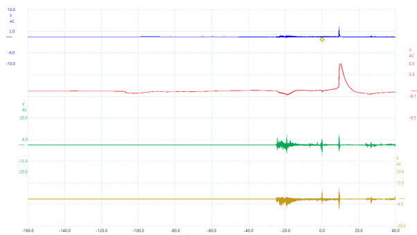
Fig. 5. Incoming signals from the filter were digitized at 20 MS/s by using four channels for fast E-field (blue plot), slow E-field (red plot), north-south magnetic field (green plot) and east-west magnetic field (gold plot)
