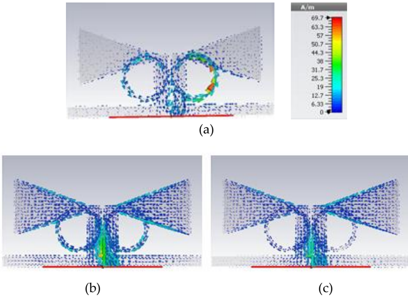
Figure 8: Vector current distribution at various frequencies: (a) 2.5 GHz, (b) 3.5 GHz and (c) 4 GHz
