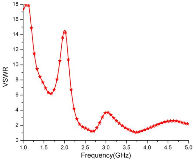
Figure 4: Simulated VSWR of proposed antenna
