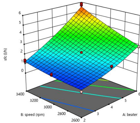
Figure 4: Effects of hammer speed and number of beaters on sfc for percentage maize milled
