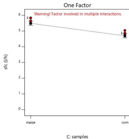
Figure 5: sfc for milling maize and guinea corn
