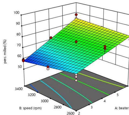
Figure 2: Effects of hammer speed and number of beaters on percentage maize milled
