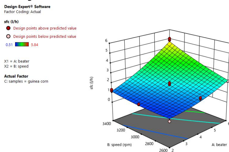
Figure 3: Effects of hammer speed and number of beaters on sfc for percentage guinea corn milled
