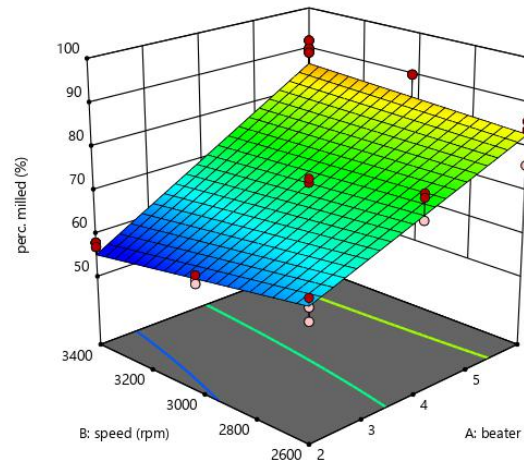
Figure 1: Effects of hammer speed and number of beaters on percentage guinea corn milled
