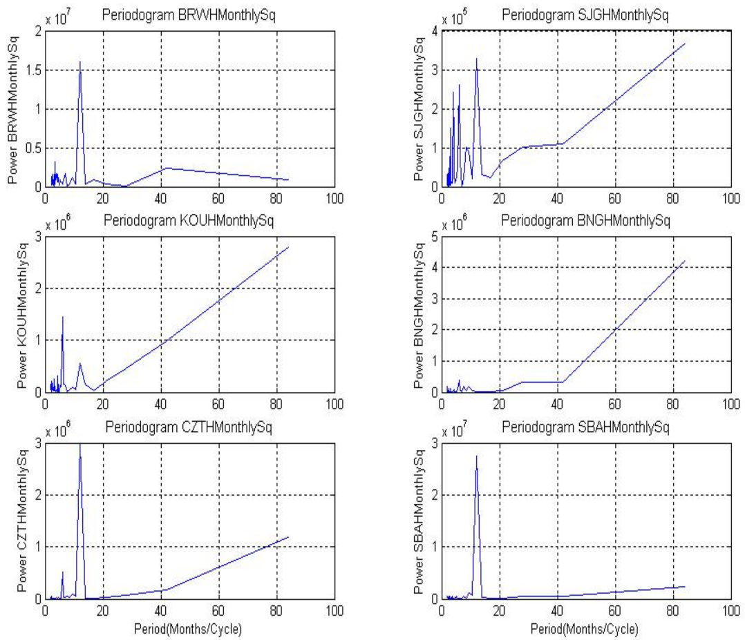
Figure 8: Periodograms showing the periods associated with Sq(H) monthly means
