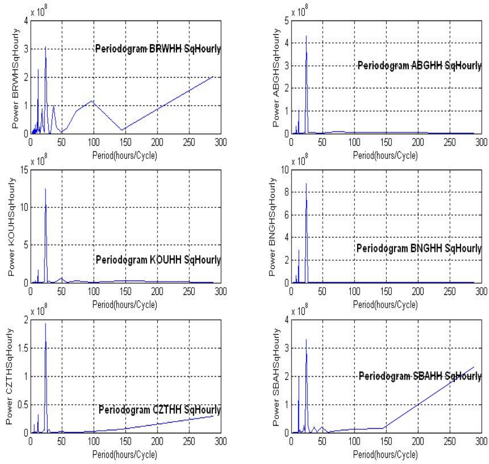
Figure 3: Periodograms showing the periods associated with Sq(H) hourly means for the year 1998
