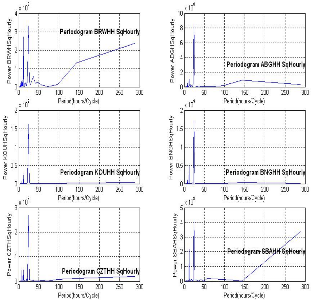
Figure 5: Periodograms showing the periods associated with Sq(H) hourly means for the year 2000
