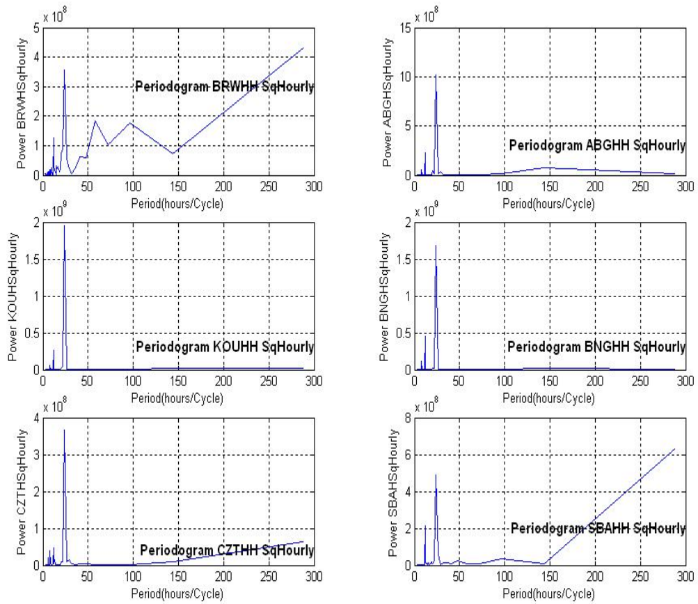
Figure 7: Periodograms showing the periods associated with Sq(H) hourly means for the year 2002
