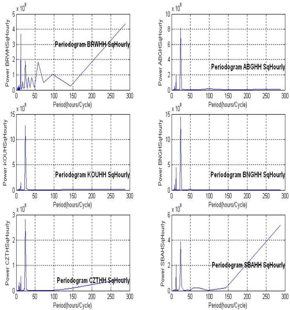
Figure 4: Periodograms showing the periods associated with Sq(H) hourly means for the year 1999
