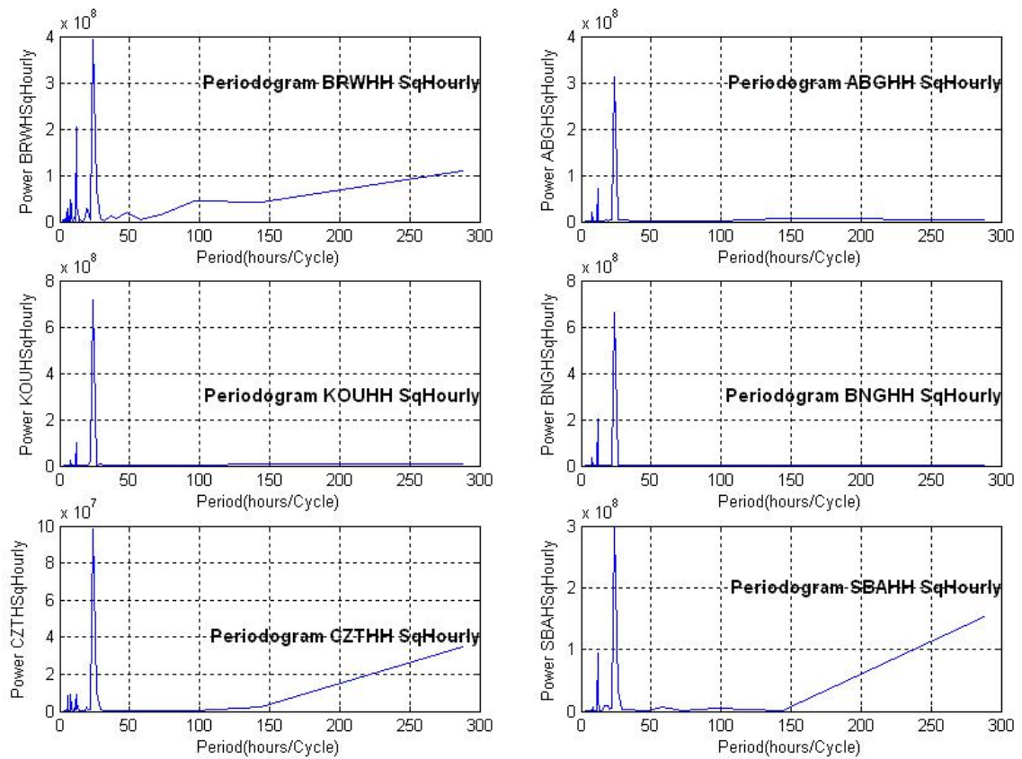
Figure 2: Periodograms showing the periods associated with Sq(H) hourly means for the year 1997
