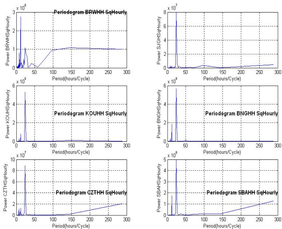
Figure 1: Periodograms showing the periods associated with Sq(H) hourly means for the year 1996
