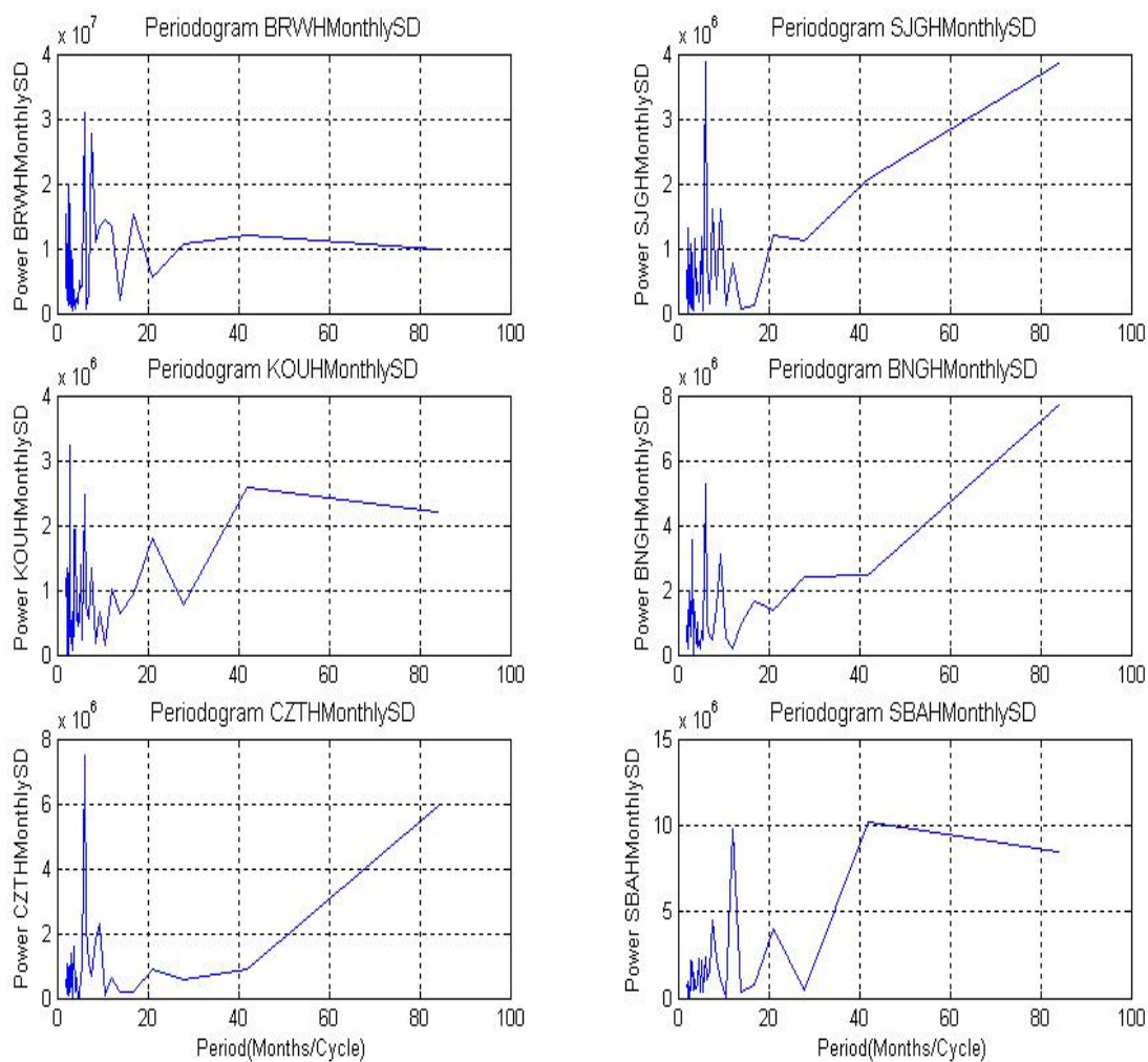
Figure 9: Periodograms showing the periods associated with SD(H) monthly means
