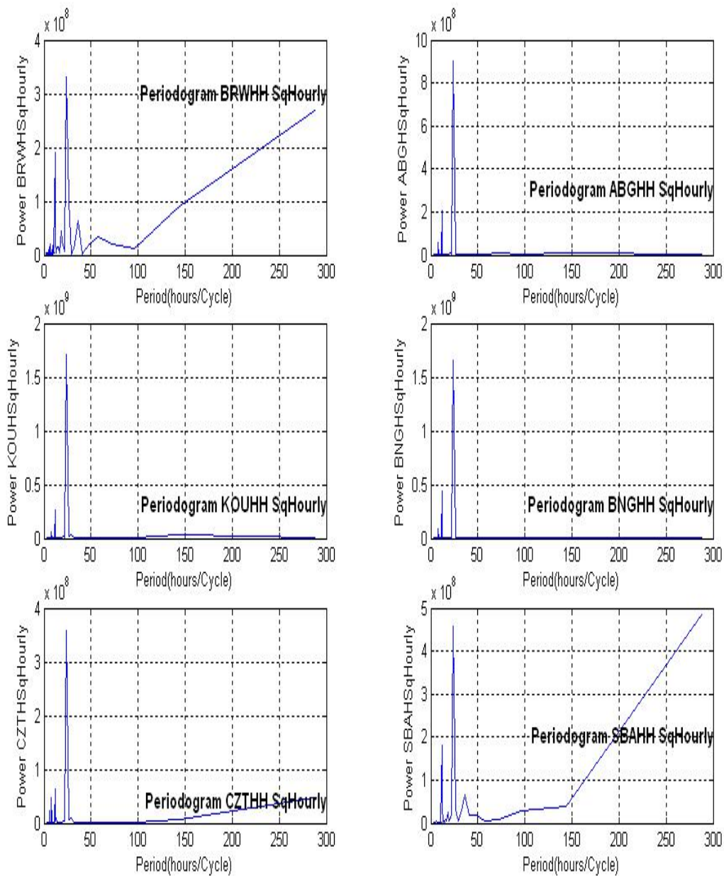
Figure 6: Periodograms showing the periods associated with Sq(H) hourly means for the year 2001
