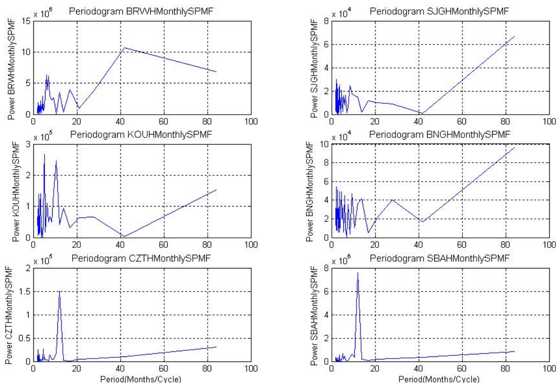
Figure 10: Periodograms showing the periods associated with SPMF (H) monthly means
