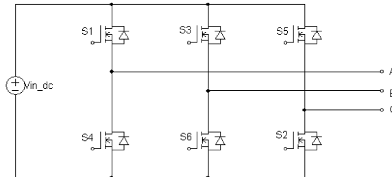
Gambar 4. Rangkaian Six-step Inverter [14]
