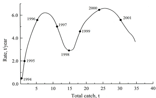
Fig. 3. Dynamic phase portrait of zander catch in Lake Vozhe (according to Tereshchenko & Zuyanova, 2006): the numbers on the curve are years of population being in the state indicated by the point on the curve
