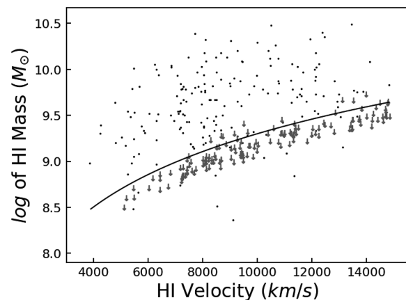
Figure 5. We show the log H I mass (uncorrected) versus H I recessional velocity for all GBT detections and non-detections released in this publication. The grey arrows indicate non-detections with the solid line being the upper limit of H I mass for these non-detections. The limit is derived from the inverse square relationship of mass and distance via our median value of M_{HI} = 10^{9.4}M_\odot being detectable at cz = 9000 km s -1 .
